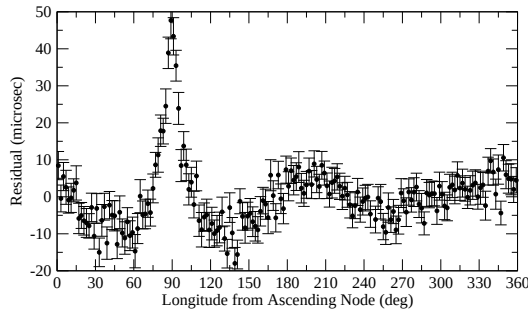
FIG. 2: The effect of the Shapiro delay caused by the gravitational potential of B seen in the timing residuals of A. The timing residuals obtained by fitting all model parameters shown in Table 1 except the Shapiro delay parameters r and s . The left-over structure represents the higher harmonics of the Shapiro delay that are unabsorbed by fits to the Keplerian parameters.
