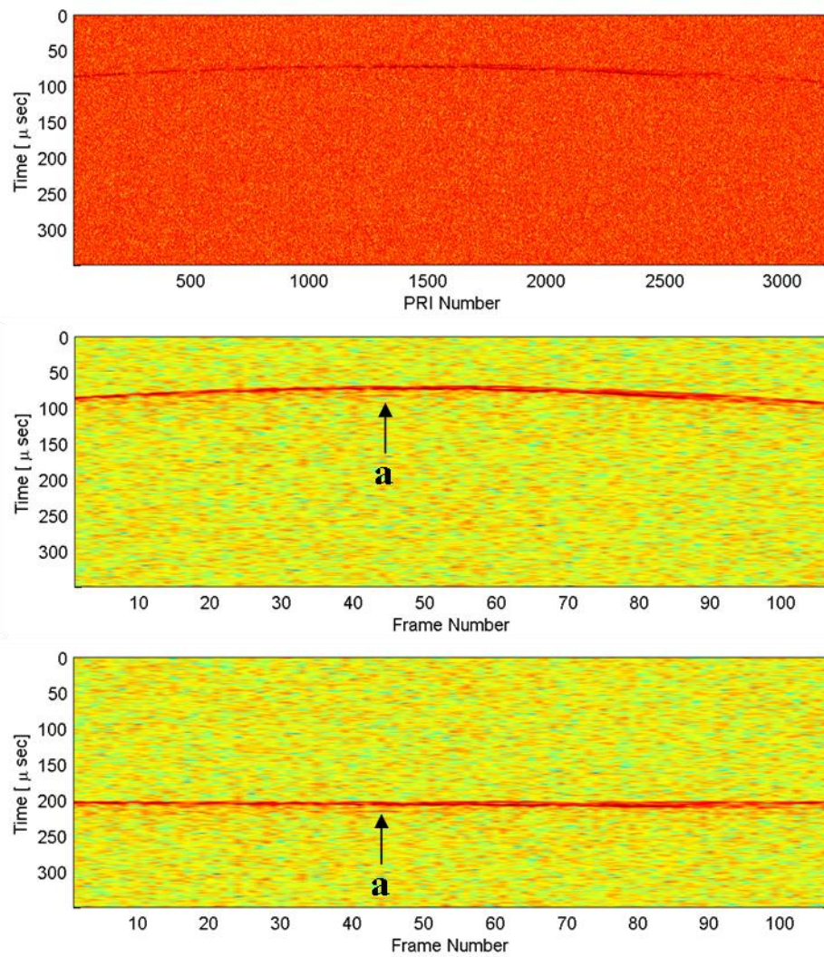
Fig. 6.3 Radargram: Phobos flyby 14-May-2015
