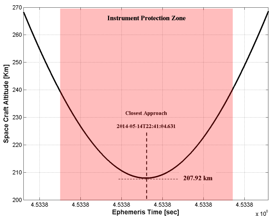
Fig. 6.1 Spacecraft altitude versus instrument protection zone
