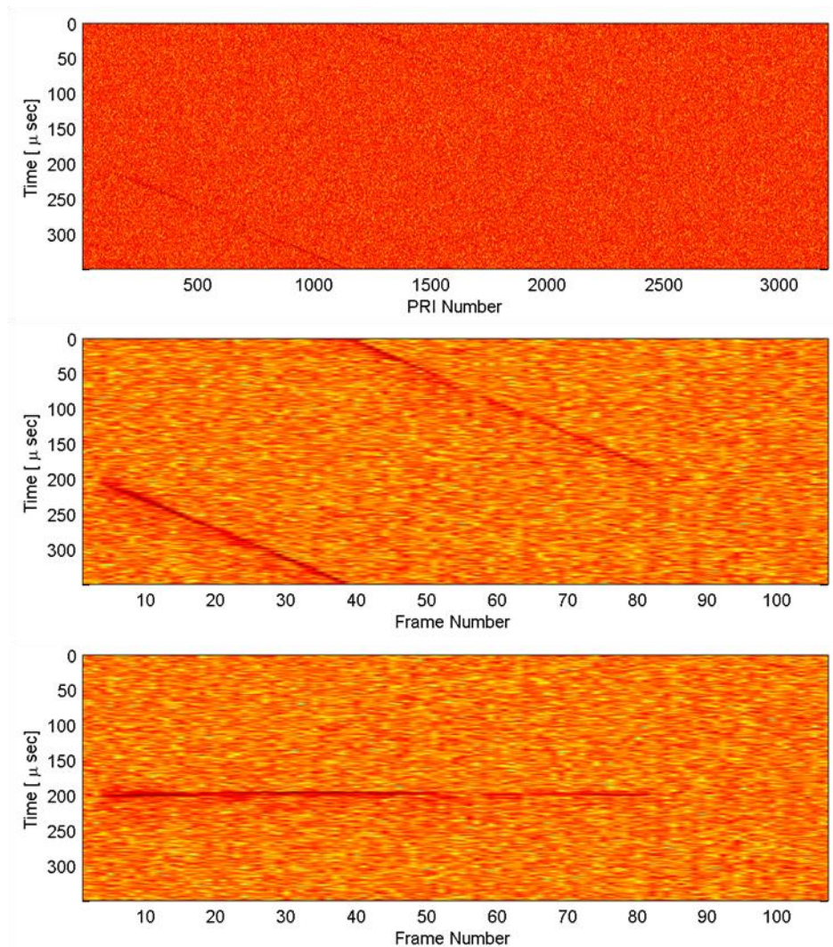
Fig. 5.6 Departure Super Frame processing results
