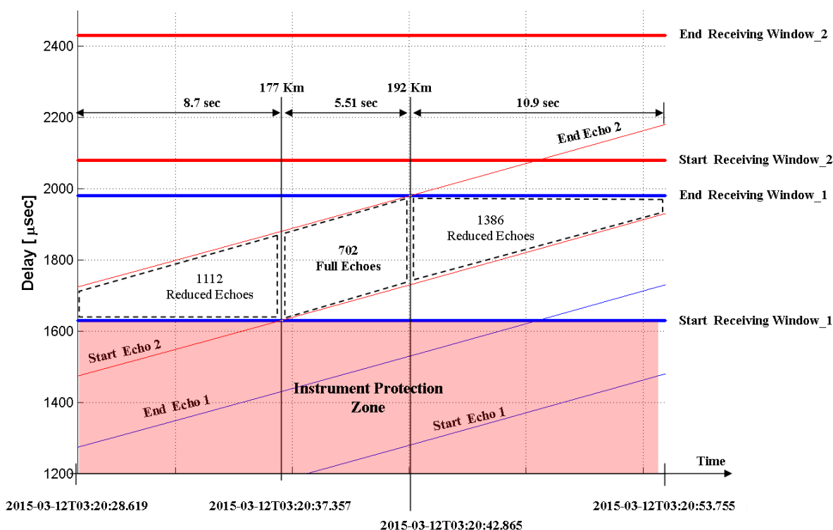
Fig. 5.4 Departure Super Frame, real observation data collection
