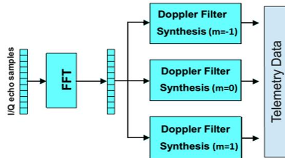
Fig. 2.5 Doppler Processing Telemetry Data
