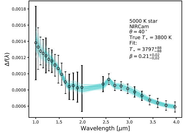
Figure 4. Example of in-transit starspot crossing flux bumps measured with the model in equation (8) and their uncertainties, for the mag K = 7.5 , K star case, in the T_\star = 3800 K, \mu -angle \theta = 40^\circ scenario without in-transit Gaussian scatter. The models in light blue represent 100 fitting models sampled from the T_\star and \beta posterior distributions. The result of the nested sampling for fitted parameters, and their 68 percent credible intervals, are indicated in the label. The model spectra were convolved with the NIRCcam filters and degraded to the same resolutions as the observations before performing the fit.
