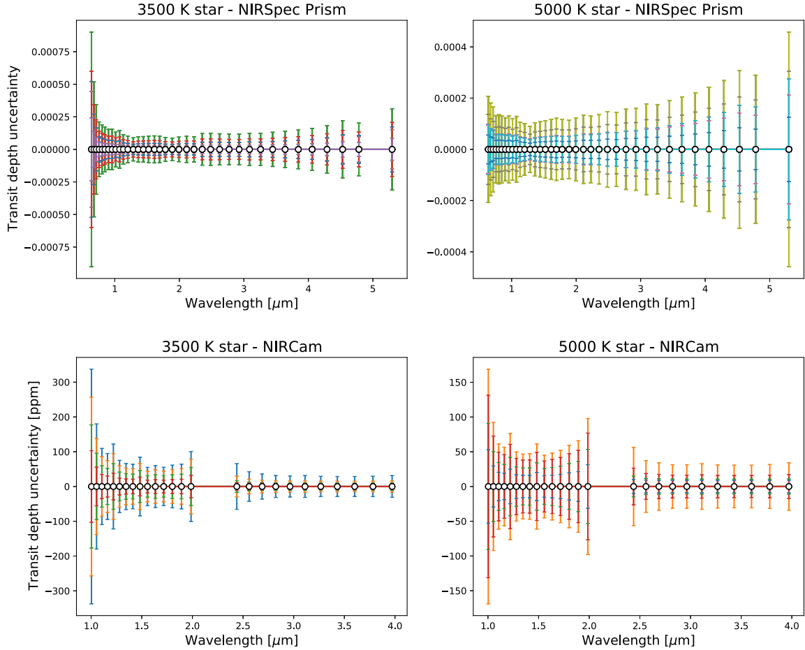
Figure 2. Transmission spectra uncertainties computed for the NIRSpec/Prism ( top ) and NIRCам/F150W2 + F322W2 ( bottom ) configurations. Increasingly larger uncertainties correspond, for NIRSpec, to mag K = 10.5, 11.5, 12.5, 13.5, and 14.5 ; for NIRCам, they correspond to K = 4.5, 6.0, 7.5, and 9.0 . M and K star scenarios are shown on the left and right column, respectively.
