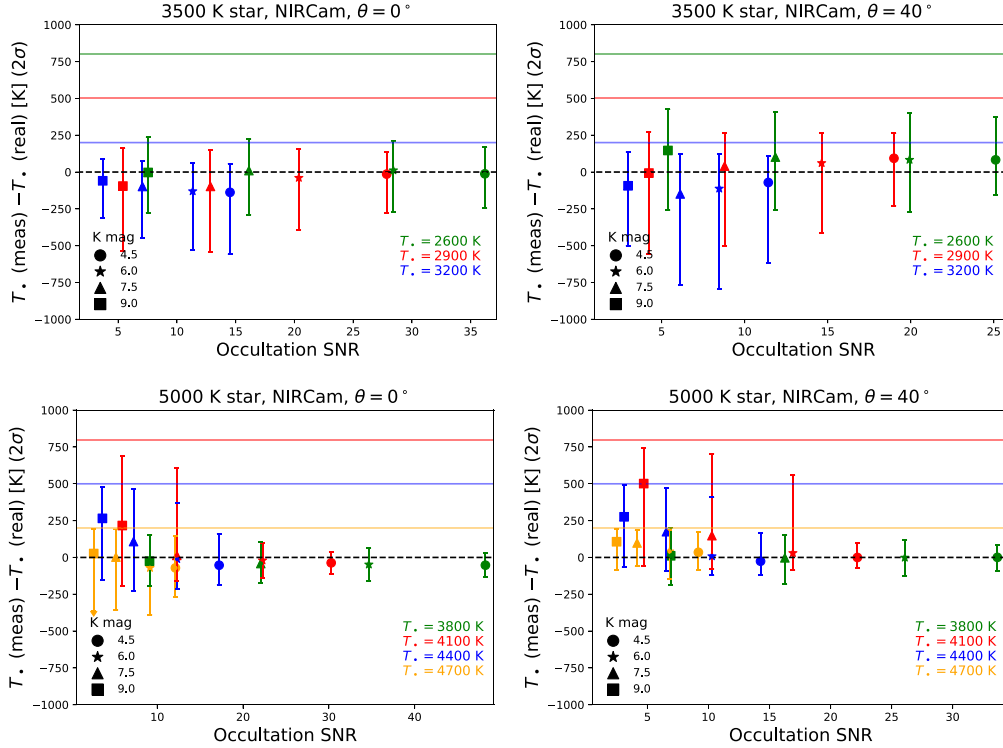
Figure 6. Same as Fig. 5, but for NIRCам/F150W2 + F322W2.
