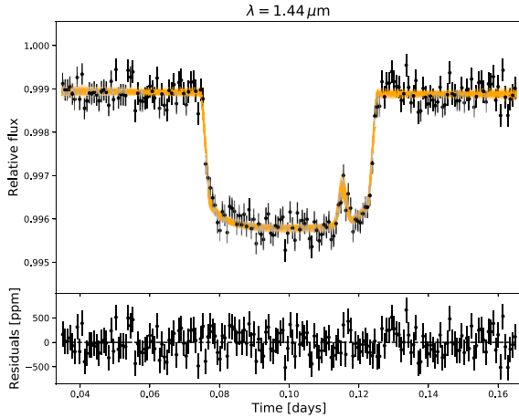
Figure 3. Simulated transit of a 0.25 R_J planet orbiting a 10.5-mag _K , 0.47 R_\odot , 3500 K star, occulting a 2900 K starspot at limb angle \theta = 40^\circ , observed with NIRSpect/Prism in the wavelength bin centred at \simeq 1.4 \mu\text{m} . This plot presents one of the noise realizations to better show the extent of the flux uncertainties. In orange on the upper panel, 300 samples from the posterior distributions obtained with the transit and Gaussian profile modelling are shown. The lower panel shows the residuals of the best-fit model, presenting a white-noise scatter, in parts per million.
