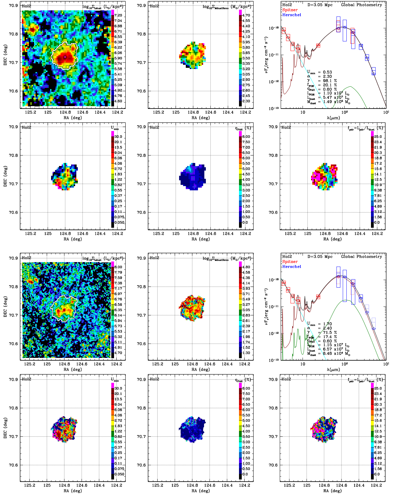
Figure 17.1 Hol2: Model results at M160 PSF (rows 1 and 2) and at S250 PSF (rows 3 and 4). Dust luminosity per area \Sigma_{Ld} (column 1, rows 1 and 3) is shown for entire field, with adopted galaxy mask boundary in white. Dust mass per area \Sigma_{Md} (column 2, rows 1 and 3) is after renormalization (see text). U_{\min, \text{DL07}} , q_{\text{PAH}} and f_{\text{PDR}} are shown in rows 2 and 4. The global SED (column 3, rows 1 and 3) is shown for single-pixel modeling, with contributions from dust heated by U_{\min} (green), dust heated by U > U_{\min} (red) and starlight (cyan); values of U_{\min} and M_d in the figure label are for the DL07 model before renormalization. Herschel (blue rectangles) and Spitzer (red rectangles) photometry is shown; vertical extent is \pm 1\sigma . Diamonds show the band-convolved flux for the model.
