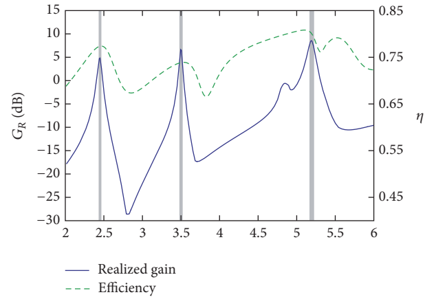
FIGURE 4: Realized gain and radiation efficiency of the designed antenna shown in Figure 1.
