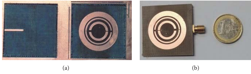
FIGURE 2: Photo of the designed antenna shown in Figure 1: (a) top and bottom layers; (b) assembled antenna.
