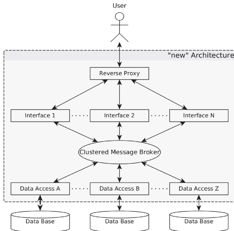
Figure 2. Revisited Architecture, skeleton diagram.
