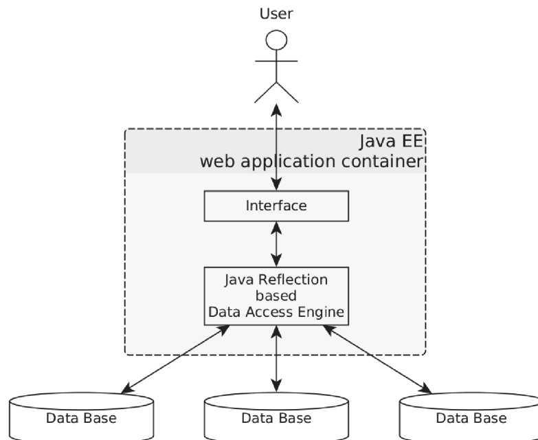
Figure 1. VO-Dance Architecture, skeleton diagram. Actually the Interface and the Data Access modules are separated only because they live in different packages with a dependency of the Interface on the Data Access . DBs can be generic ones, once a suitable SQL implementation is provided in the code, but Java is set as the only possible language for coding such differentiation.
