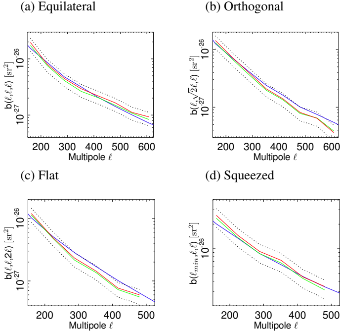
Fig. 14. Bispectra of the NILC (green) and MILCA (red) y -maps for four different configurations (equilateral, orthogonal, flat and squeezed), compared with the bispectrum of the projected map of the PSZ2 clusters (blue). \pm 1\sigma uncertainties are indicated as black dotted lines.
