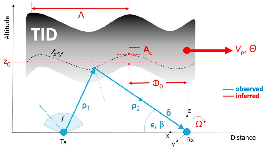
Figure 2. Traveling ionospheric disturbance (TID) model as a perfectly reflecting corrugated mirror (dashed line) moving across the area (red arrow) and causing variations of the oblique-incidence signal (blue line) characteristics \{\rho(t), \delta(t), \epsilon(t), \text{ and } \beta(t)\} .
