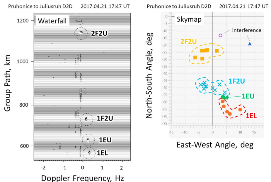
Figure 4. Digisonde-to-Digisonde (D2D) measurements for northern Pruhonice to Juliusruh link, f = 5.05 MHz; Doppler waterfall and skymap.
