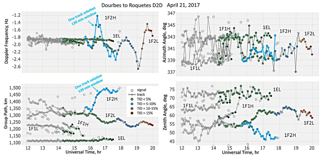
Figure 7. Automatically tracked signal parameter for the 1,083 km DB → EB link: Doppler frequency, group path length, and azimuth and zenith angles. DB = Dourbes; EB = Ebro; D2D = Digisonde-to-Digisonde.
