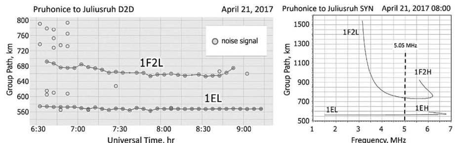
Figure 6. (left) Automatically tracked signal group path tracks for the 512 km PQ \rightarrow JR (5.05 MHz) link. (right) The synthesized oblique ionogram for 08:00 UT. JR = Juliusruh; PQ = Pruhonice; D2D = Digisonde-to-Digisonde.
