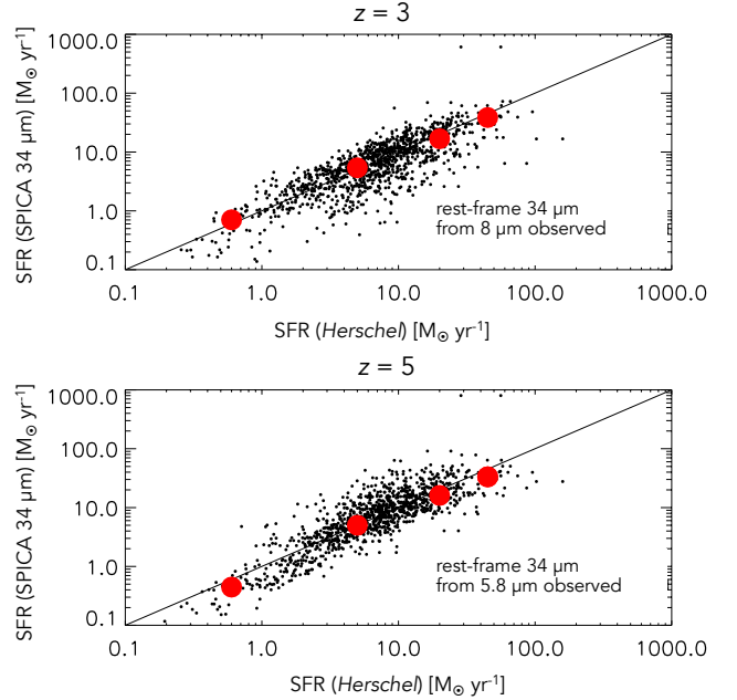
Figure 4. Examples of how the photometric SPICA survey at 34 \mu\text{m} could be able to recover the SFR of star-forming galaxies at z=3 and z=5 . We compare the SFR (effectively the total IR luminosity) extrapolated from the observed 34- \mu\text{m} flux density at z=3 (top panel) to that computed when including photometric data from Herschel . To perform this test we used a sample of local galaxies ( z < 0.3 ) from the COSMOS survey (Laigle et al. 2016), where the observed 8- \mu\text{m} IRAC fluxes mimic the rest-frame emission of the 34- \mu\text{m} filter at z=3 . Similarly, we adopted the 5.8- \mu\text{m} IRAC fluxes (bottom panel) to probe the 34- \mu\text{m} filter at z=5 . The red filled circles show the median values in bins of SFR.
