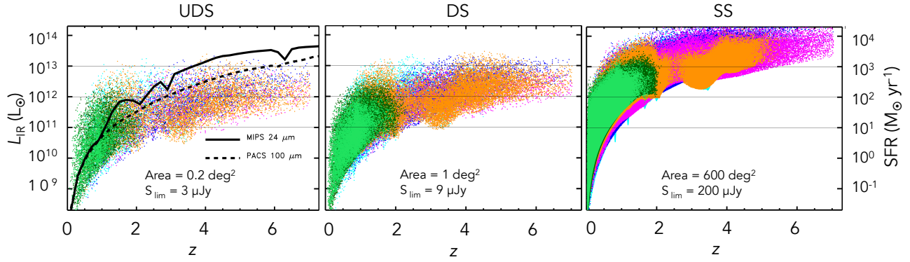
Figure 7. Expected total IR luminosity (SFR) as a function of redshift for the three photometric surveys planned with SPICA-SMI/CAM (left: UDS to 3\mu\text{Jy} ; middle: DS to 9\mu\text{Jy} ; right: SS to 0.2\text{mJy} ). The different colours of the points represent the behaviour of different SED-types: cyan, starburst ; green, spiral ; dark-green, SF-AGN(spiral) ; orange, SF-AGN(SB) ; magenta, AGN2 ; and blue, AGN1 (see Gruppioni et al. 2013 for details and the text for a brief description of these populations). For comparison, the limiting IR luminosity corresponding to the fluxes reached by the deepest surveys with Spitzer (MIPS 24\mu\text{m} ) and Herschel (PACS 100\mu\text{m} ) are shown in the left panel as black solid and dashed lines respectively. The horizontal lines mark the LIRG, ULIRG and HyLIRG limits.
