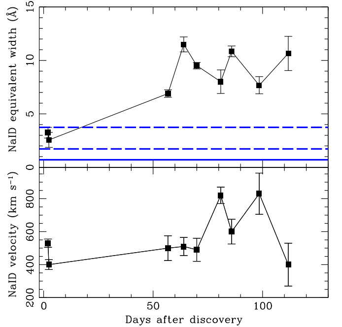
Figure 8. Top: the absorption near the Na I D equivalent width evolution with time for SN 2011A. The solid blue line shows the average Na I D EWs (averaged over time) for all CSP SNe II (including SNe IIn, but not SNe IIb) where the EW is most likely of ISM origin. The lower dashed blue line shows the 1\sigma error on the EW estimation, and the upper shows the 3\sigma error. The lower panel shows the absorption near the Na I D velocity evolution measured with respect to the emission.
