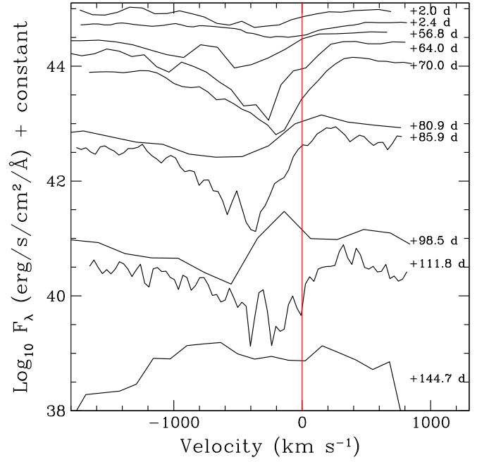
Figure 7. Zoom on the absorption near Na I D of our SN 2011A optical spectra. The epochs are listed with respect to the discovery date (2011 January 2.30 UT = 0 days). The red line represents the center of the Na I D corrected to the redshift of the host galaxy. We note that this appears offset by \sim 200 km s^{-1} from the emission component of Na I D.
