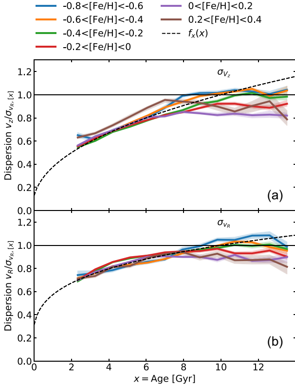
Figure 6. Same as Fig. 5 but for stars lying in different [\text{Fe}/\text{H}] bins. For older stars the profiles show a mild variation with [\text{Fe}/\text{H}] .
