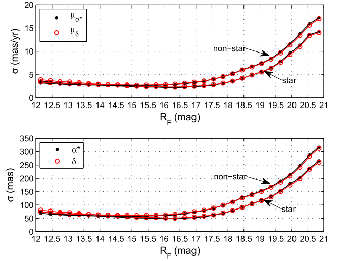
Figure 9. Mean formal errors of APOP absolute proper motions ( \mu_{\alpha*}, \mu_\delta ) and positions ( \alpha, \delta ) of stars and non-stars as a function of R_F magnitude. The magnitude is binned in 0.3 mag bins, with at least 100,000 objects per bin. The marker * in the \mu_\alpha indicates multiplication by \cos(\delta) . Top: the formal errors of absolute proper motions in \text{mas yr}^{-1} ; bottom: the formal errors of positions in mas.
