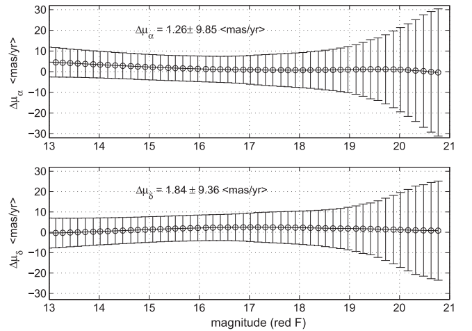
Figure 17. Mean and dispersion (rms) of the proper motion differences between APOGEE and PPMXL as a function of magnitude.
