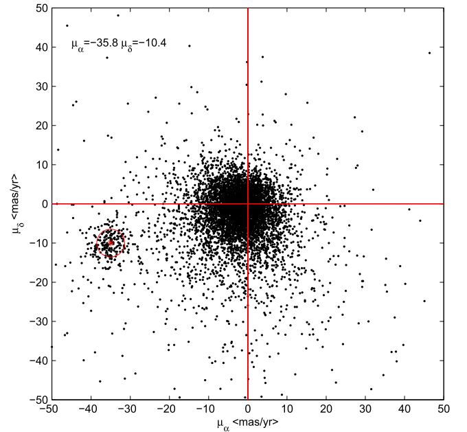
Figure 19. Proper motion vector-point diagram for all the objects in APOP with magnitude R_F < 18.0 in the area of the Praesepe cluster. A tight group at \mu_{\alpha*} = -35.8 \text{ mas yr}^{-1} , \mu_\delta = -10.4 \text{ mas yr}^{-1} indicates the location of Praesepe and permits a segregation between the cluster and field stars. In addition, this value is quite close to the Hipparcos data for Praesepe , which is \mu_{\alpha*} = -35.81 \text{ mas yr}^{-1} , \mu_\delta = -12.85 \text{ mas yr}^{-1} (van Leeuwen 2009).
