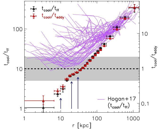
Figure 11. Cooling time normalized to the freefall time ( t_{\text{cool}}/t_{\text{ff}} ; black) and to the eddy time ( t_{\text{cool}}/t_{\text{eddy}} ; red) as a function of radius for the Phoenix cluster. These ratios have been used as predictors for the growth of thermal instabilities (e.g., Gaspari et al. 2012, 2018; McCourt et al. 2012; Sharma et al. 2012; Voit et al. 2015), where the denominator is meant to roughly approximate the mixing time of the gas. Here, the freefall time has been calculated using the strong lensing model model, described in Section 2.1, while the eddy timescale has been computed assuming a line of sight turbulence of 250 \text{ km s}^{-1} and a bubble diameter of 20 \text{ kpc} (see Equation (5) in Gaspari et al. 2018). We show, for comparison, 57 clusters from Hogan et al. (2017), for which the t_{\text{cool}}/t_{\text{ff}} ratio has been computed with careful consideration of the gravitational potential due to both the cluster and the central galaxy. The Phoenix cluster is an obvious outlier in the t_{\text{cool}}/t_{\text{ff}} space, as the only known cluster reaching a value of unity in the core. The dotted black line and shaded gray region highlights the condensation threshold for these two ratios. This figure demonstrates that thermal instabilities are likely to develop within the central 30 \text{ kpc} , where we see a significant amount of cool gas.
