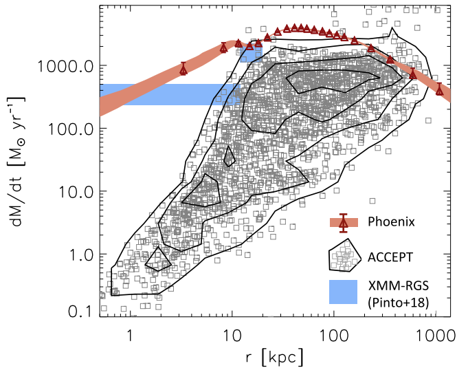
Figure 14. Classical cooling rate as a function of radius, defined following Equation (7). Gray squares show profiles for 91 cool core clusters in the ACCEPT sample (Cavagnolo et al. 2009), resampled to a common binning. Black contours show the distribution of these profiles, which is relatively flat at r \gtrsim 30 kpc, and steeply declining at interior radii. This rapid decline in the cooling rate at the center of the cluster is prime evidence that AGN feedback is effectively preventing cooling at these radii. Red points and the shaded red curve show the cooling rate profile for the Phoenix cluster, which is significantly flatter than the median cool core profile, with a central cooling rate elevated by a factor of \sim 10^3 above the typical low- z cluster. Blue-shaded regions show the XMM-RGS spectroscopic cooling rates from Pinto et al. (2018), where we have converted temperature bins into radial bins using the three-dimensional temperature profile from Figure 8. These data further support the picture in which cooling is proceeding with relatively little impedance at the center of the Phoenix cluster.
