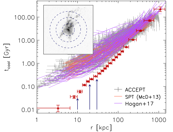
Figure 10. Cooling time as a function of radius for the Phoenix cluster (red points). We show, for comparison, 91 cool core clusters in the ACCEPT sample (Cavagnolo et al. 2009), 57 cool core clusters from the sample of Hogan et al. (2017), and 27 high- z cool core clusters from McDonald et al. (2013b). In the inset, we show the [O II] image of the central galaxy, with radii of 10, 20, and 30 kpc depicted as dashed circles. These radii are also highlighted in the profile, showing that the bulk of the cool gas is present at radii where the cooling time is \lesssim 100 \text{ Myr} . At these radii, the Phoenix cluster has the shortest cooling time of any known cluster by a substantial margin.
