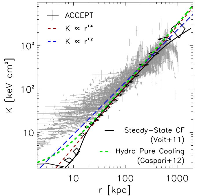
Figure 9. Three-dimensional entropy profile for the Phoenix cluster (black diamonds). This profile was derived based on the best-fit three-dimensional density and temperature models, shown in Figure 8. In gray, we show entropy profiles for 91 cool core clusters ( K_0 < 30 \text{ keV cm}^2 ) in the ACCEP sample (Cavagnolo et al. 2009). In blue, we show the canonical K \propto r^{1.2} “baseline entropy profile” from Voit et al. (2005), while in red and black we show the simple and more complicated (respectively) predictions for a steady-state cooling flow with \dot{M} \sim 3000 M_\odot \text{ yr}^{-1} , following (Voit 2011). In green, we show the prediction for a pure-cooling flow from hydrodynamic simulations (Gaspari et al. 2012). We note that, at all radii, the data for the Phoenix cluster lies between the simulation and analytic theory predictions for a pure-cooling flow. This plot demonstrates the uniqueness of the Phoenix cluster, which exhibits no evidence for a break at small radii (e.g., Panagoulia et al. 2014; Babyk et al. 2018) and with a central entropy lying roughly an order of magnitude below any other cluster known.
