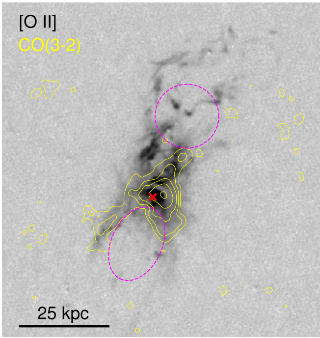
Figure 17. [O II] map of the inner \sim 50 kpc of the Phoenix cluster. Overlaid on this map are contours showing the CO(3–2) emission, from Russell et al. (2017), and the locations of the X-ray cavities, shown as magenta ellipses. This figure demonstrates that the bulk of the cool, multiphase gas is either behind, or draped around, the bubbles. However, a small fraction of the multiphase gas leads the bubbles, extending for \sim 20 kpc beyond the leading edge of both the northern and southern bubbles.
