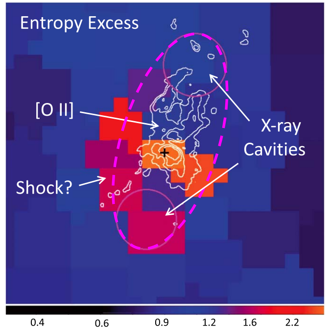
Figure 16. Excess entropy map, produced by dividing the two-dimensional entropy map (Figure 12) by the prediction for a steady, homogeneous cooling flow (see Figure 9). Overplotted are the X-ray cavities (magenta circles), the location of the X-ray AGN (black cross), and the highest surface brightness [O II] emission (white contours). We also show, for illustrative purposes, a magenta ring at the location that we think there may be a cocoon shock. This ring is coincident with a ring of high-entropy gas, where the entropy (and cooling time) is elevated compared to the predictions from the simple cooling flow model.
