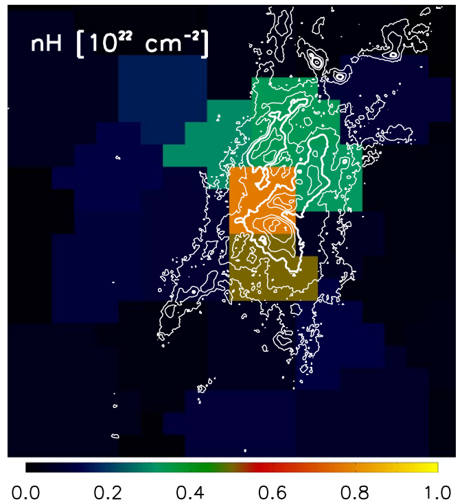
Figure 7. Two-dimensional X-ray absorption map for the inner \sim 25 kpc of the Phoenix cluster. Overlaid in white are the contours of constant [O II] surface brightness, where we have highlighted the highest surface brightness emission with a thicker contour. This figure demonstrates that the X-ray-absorbing material is cospatial with the cool, line-emitting gas.
