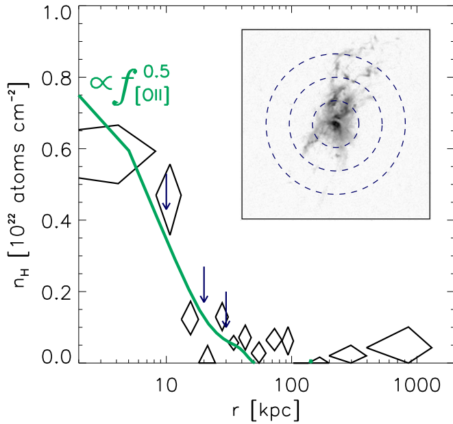
Figure 6. This figure shows the inferred photoelectric absorption in the X-ray due to cool gas within the Phoenix cluster as a function of radius. We find relatively strong absorption in the inner \sim 10 kpc, which falls off quickly to become negligible at r \gtrsim 50 kpc. For comparison, we show the radial profile of the absorbing column (green) as inferred from the [O II] map (shown in grayscale). Assuming that the [O II] emission roughly traces the gas doing the absorbing, then the absorbing column should be proportional to the square root of the emission-line luminosity, which qualitatively appears to provide a good fit to the data. Further, integrating the total amount of X-ray absorption over the volume of absorbing material yields a total gas mass similar to that of the cold molecular gas (Russell et al. 2017). In the inset, we show the [O II] image of the inner \sim 40 kpc, with annuli overlaid at 10, 20, and 30 kpc. These radii are marked in the radial profile with arrows.
