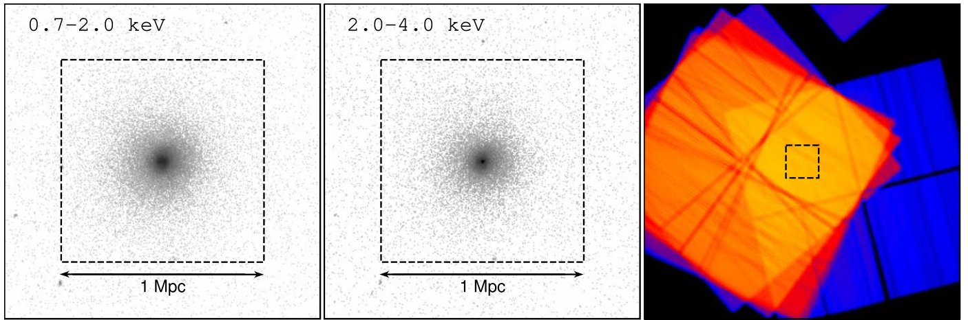
Figure 3. Left: 0.7–2.0 keV counts image for the inner \sim 1 Mpc of the Phoenix cluster, combining data from 12 observations totaling 551 ks. This soft X-ray image shows a relaxed (circular) cluster with a strong cool core. There is no evidence for a central point source at these energies. Middle: 2.0–4.0 keV counts image for the same region as shown in the left panel. This hard-band image shows evidence for a central point source, embedded at the center of a strong cool core. The absence of this source in the soft band indicates a highly obscured AGN. Right: combined exposure map for all 12 observations, with the size of the region from the left panels shown as a small square. This image highlights that all of the relevant data for our analysis (i.e., inner \sim 1500 kpc) comes from a small region near the ACIS-I aim point, where we have uniform coverage over all 12 exposure. The bulk of the remaining three ACIS-I chips were used as background regions for spectroscopic analyses.
