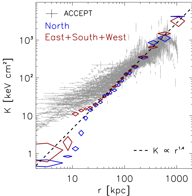
Figure 13. Three-dimensional entropy profile extracted along a northern wedge ( 90^\circ opening angle, tilted west by 10^\circ to match the position angle of the jet) and along the remaining 270^\circ . These profiles show that the area surrounding the low-entropy filament in Figure 12 is similar to a “typical” cool core cluster, with a shallower entropy profile between 10 < r < 50 kpc than at larger radii. At r < 10 kpc, and along the northern filament, the entropy profile drops dramatically, indicating the onset of thermal instabilities.
