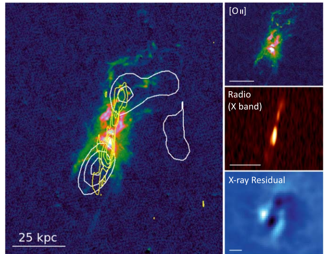
Figure 5. On the left, we show the continuum-subtracted [O II] emission map, with radio (yellow) and X-ray (white) contours overlaid. For the X-ray contours, we only show the significant negative residuals, after a two-dimensional model has been subtracted from the large-scale emission (see Section 2.2.3). In the right panels, we show the [O II] (top), radio (middle), and X-ray (bottom) images individually. X-ray images have been shifted by a half pixel to align the optical and X-ray nuclei. This figure demonstrates the near-perfect correspondence between the radio jets, X-ray cavities, and cool filaments. The jets appear to be responsible for inflating bubbles in the hot gas, while the cool gas appears draped around and behind the resulting cavities. We will discuss this further in Section 4.3.
