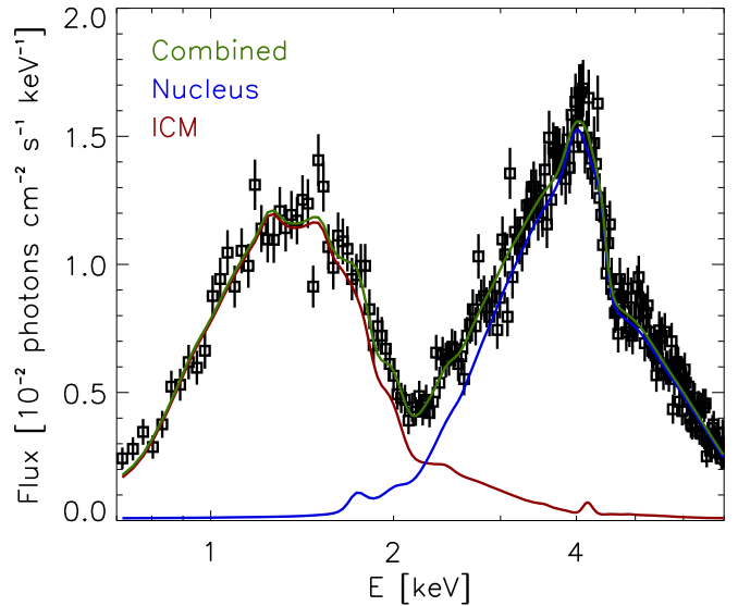
Figure 4. Observed-frame X-ray spectrum of the inner 1''.5 of the Phoenix cluster. This spectrum is dominated at < 2 keV by thermal plasma with kT \sim 2 keV, with a small amount of both intrinsic and Galactic absorption (red curve). At > 2 keV, the spectrum is dominated by a heavily obscured, marginally piled up central point source, which is well modeled by the MYTORUS model (blue curve; Murphy & Yaqoob 2009). This model has been used, in conjunction with Chandra ray tracing software, to produce a model of the point-source emission for each OBSID, which is used to determine the underlying thermal emission at all radii.
