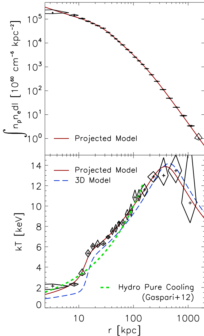
Figure 8. Top: projected X-ray emissivity per unit area for the Phoenix cluster. In red, we show the best-fit three-dimensional model (Equation (1)), projected onto two dimensions. This model provides an excellent fit to the data at all radii and reveals a strongly peaked cool core cluster. Bottom: projected X-ray temperature profile for the Phoenix cluster. In red, we show the best-fit three-dimensional model (Equation (2)), projected onto two dimensions. In blue, we show the true three-dimensional model, which is slightly cooler in the center and slightly hotter at large radii than the projected profile. In green, we show the prediction for the inner 150 kpc from hydrodynamic simulations for a pure-cooling flow ( T \propto r^{1/2} ; Gaspari et al. 2012). Given the shape of the mass profile over the radial range considered here, this curve is consistent with kT(r) \propto GM(<r)/r . Phoenix exhibits the strongest falloff in temperature of any cluster known, going from a peak temperature of \sim 14 keV to a minimum of \sim 1 keV in the two innermost bins ( r \lesssim 10 kpc), consistent with the expectations for pure cooling. The temperature profile appears to have two regions: the larger scale cool core with a temperature of \sim 6 keV and a size of \sim 50 kpc, and a smaller, cooler region with a temperature of \sim 1 keV and a size of \sim 10 kpc.
