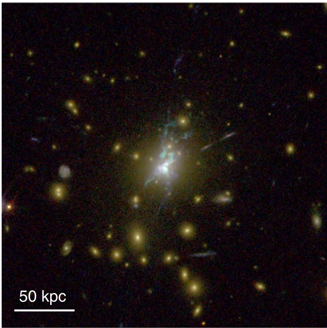
Figure 1. HST ACS-WFC2 color image of the core of the Phoenix cluster, made by combining images in the F475W, F775W, and F850LP bands. This image shows a giant elliptical central galaxy with a morphologically complex, dusty starburst component that extends for \sim 50 kpc to the north and south. Previously identified (McDonald et al. 2015) linear filaments to the north and northwest, which extend for \sim 100 kpc, have been spectroscopically identified as radial arcs (see Section 2.1).
