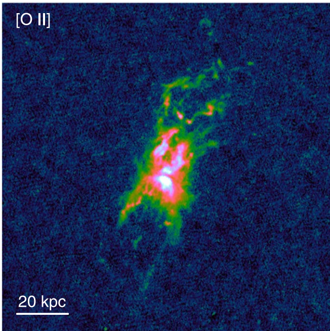
Figure 2. Continuum-subtracted [O II] \lambda\lambda 3726, 3729 image of the central galaxy in the Phoenix cluster. This image was generated by subtracting a continuum model, based on the three color images in Figure 1, from an image in the narrowband FR601N filter, as described in Section 2.1. This image reveals a significantly more complex network of emission-line filaments than seen in previous ground-based emission-line maps (McDonald et al. 2014). The bulk of the emission is contained in the inner \sim 20 kpc, with morphologically complex filaments extending as far as \sim 40 kpc to the south and \sim 60 kpc to the north. In general, the emission is confined to a relatively narrow range of position angles, slightly west of north, corresponding to the direction of previously identified bubbles in the X-ray (Hlavacek-Larrondo et al. 2015).
