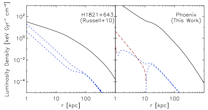
Figure 15. Luminosity (cooling rate) per particle as a function of radius for the H1821+643 (left) and Phoenix (right) clusters. In black, we show the cooling rate due to thermal bremsstrahlung emission, based on the measured density and temperature profiles. The dotted blue (red) curves show the Compton cooling (heating) rate as a function of radius, where the upper curve is for a typical unobscured QSO spectrum, while the lower curve is for a typical obscured QSO spectrum (Sazonov et al. 2004). This figure demonstrates that, while Compton cooling is important for the lower-mass H1821+643 cluster, it is likely not contributing in a meaningful way to the thermodynamics at the center of the Phoenix cluster.
