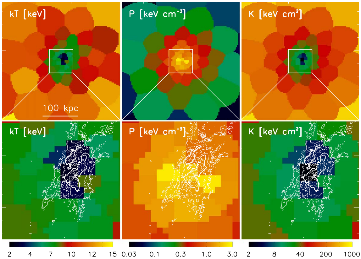
Figure 12. Thermodynamic maps, showing temperature (left), pressure (middle), and entropy (right). Images are 330 \times 330 kpc (top) and 66 \times 66 kpc (bottom) on a side. In the lower panels, we show contours of constant [O II] surface brightness, highlighting the location of the cool, line-emitting gas. We highlight the highest surface brightness emission with a thick white contour. Both the temperature and entropy profiles show a filament of cool, low-entropy gas to the north, extending \sim 20 kpc. This asymmetric low-entropy region, which is also the location of the strongest X-ray absorption (see Figure 7) is cospatial with the cool, line-emitting gas. This region appears to be in, or close to, pressure equilibrium with the surrounding regions. There is some weak evidence for enhanced pressure to the east and west, which is primarily driven by an increase in density (i.e., the accompanying temperature increase is mild).
