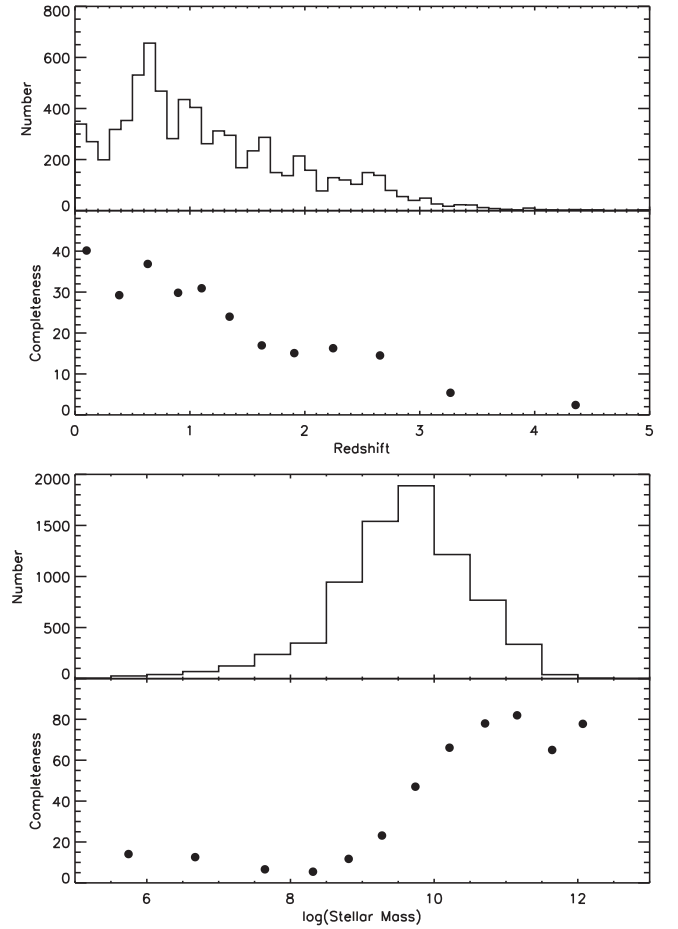
Figure 1. Redshift (top) and stellar mass (bottom) distributions and completeness. The completeness indicates the percentage of galaxies in each bin that satisfy the magnitude cut ( H < 24.5 ) and are observed to at least the 2-epoch depth in the H -band.
