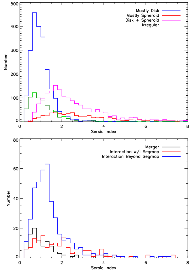
Figure 12. Sérsic index for visually classified galaxies in GOODS-S color coded by their main morphology class (top) and the interaction class (bottom). The main morphology classes are further refined by their relative diskiness/bulgeiness, into “Mostly Disk” ( >2/3 classifiers call it a disk and <2/3 classifiers call it a spheroid), “Mostly Spheroid” ( >2/3 classifiers call it a spheroid and <2/3 classifiers call it a disk), “Disk + Spheroid” ( >2/3 classifiers call it a disk and >2/3 classifiers call it a spheroid) and “Irregular” ( >2/3 classifiers call it irregular, <2/3 classifiers call it a disk, and <2/3 classifiers call it a spheroid).
