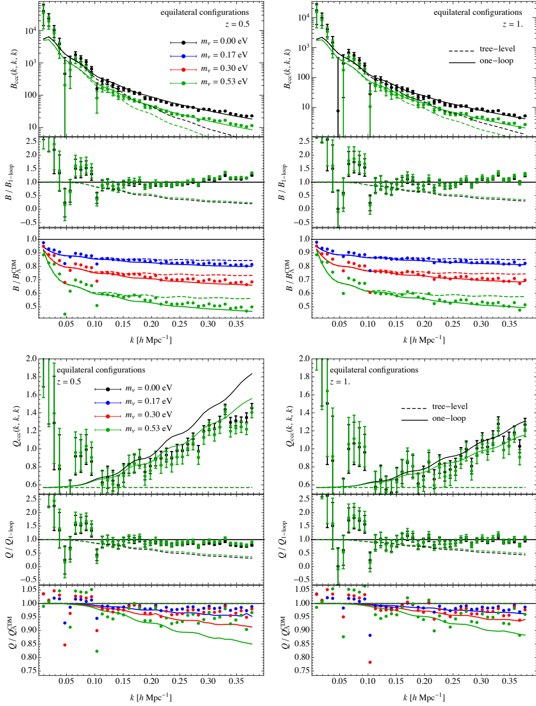
Figure 3. Top panels: equilateral configurations of the cold matter bispectrum, B_{ccc}(k, k, k) , compared with tree-level (dashed curves) and one-loop (continuous curves) predictions in PT. Bottom panels: same comparison for the reduced cold matter bispectrum Q_{ccc}(k, k, k) . Left panels show the results at z = 0.5 , right panels at z = 1 . In addition to the measurements of B or Q , we plot the residuals with respect to the one-loop predictions (middle panel) and the ratio between the m_\nu \neq 0 cosmologies to the corresponding massless neutrino case (bottom panel).
