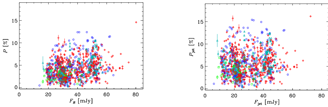
Figure 18. Left: The observed degree of polarisation as a function of the observed R -band flux density. Right: The same plot after correcting for the host contribution.
