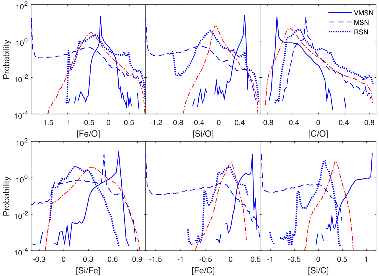
Figure 2. Probability distribution of PopIII-dominated GRBIIIs given only one abundance ratio (from left to right and top to bottom, it is [\text{Fe}/\text{O}] , [\text{Si}/\text{O}] , [\text{C}/\text{O}] , [\text{Si}/\text{Fe}] , [\text{Fe}/\text{C}] and [\text{Si}/\text{C}] ) in model VMSN (solid blue lines), MSN (dashed blue lines) and RSN (dotted blue lines). As a reference, the PDF of PopII-dominated GRBIIIs is shown as dash-dotted red line in each panel. Note that the PDFs are normalized by the total rate in each class i and therefore, in number, PopII-dominated GRBIIIs overwhelm the distribution of PopIII-dominated ones.
