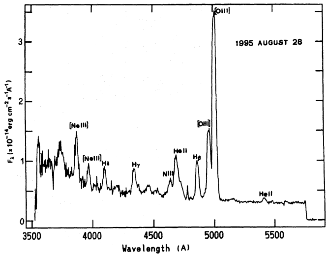
Fig. 2. The spectrum at 1283 days after maximum, is characterized by the fall of the general degree of ionization. With a few exceptions, most of the lines have become weaker than Hβ and are barely perceptible. The [O III] line at 5007Å, with intensity 5.67 relative to Hβ, appears now, on objective prism spectra, the strongest feature after Hα
