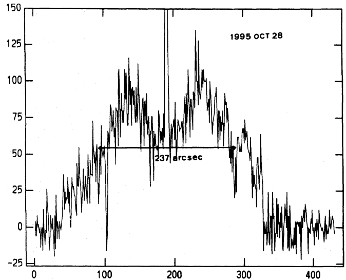
Fig. 6. Evidence of an extensive emission nebula around the nova found by scanning perpendicularly to the dispersion an H\alpha spectrum of the nova taken on 1995 October 28
