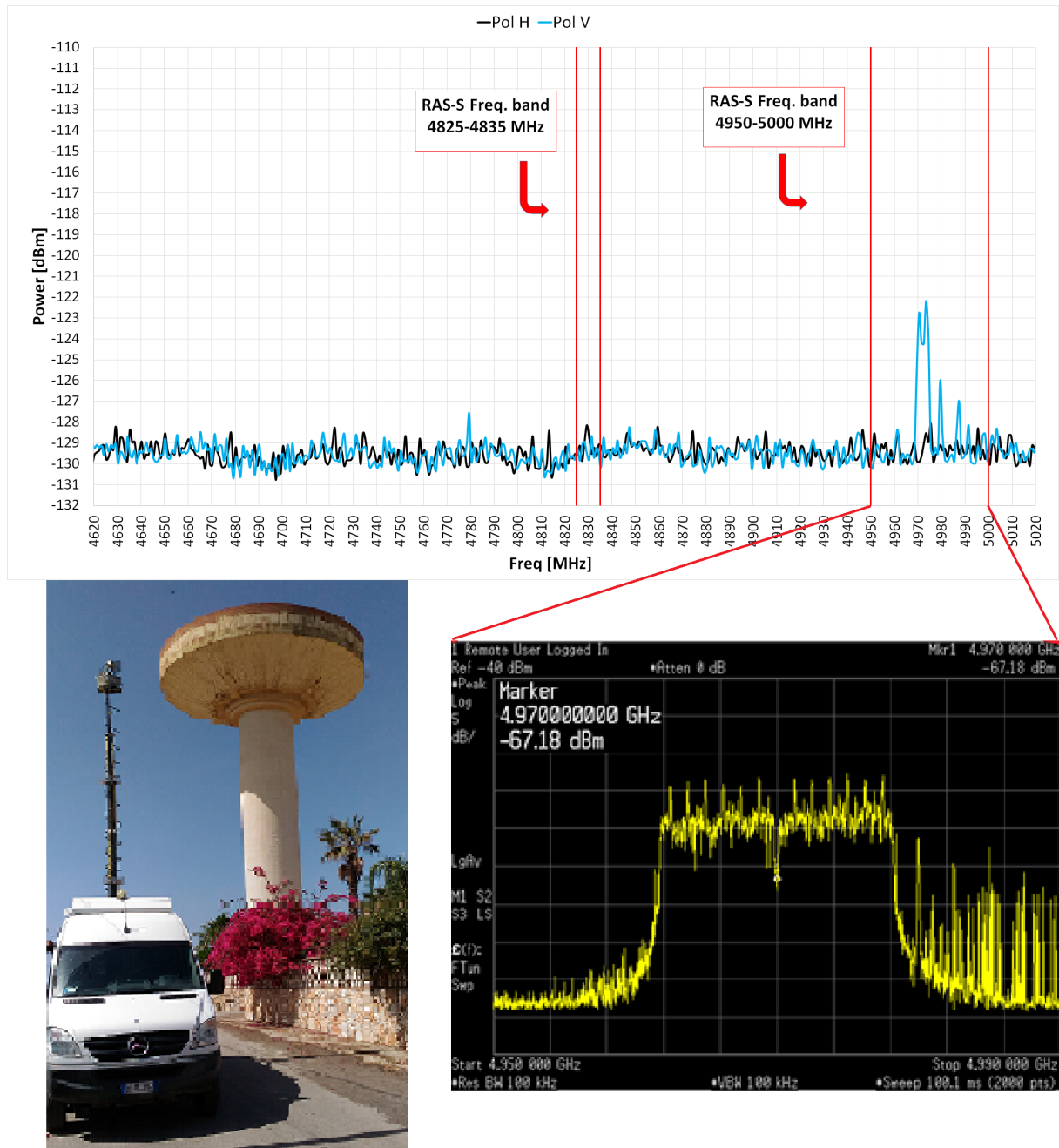
Figure 4: C-low spectra acquired during the 2016 RFI monitoring campaign at Noto (top panel). The two H- (black line) and V- (light blue line) polarized spectra were acquired with a panoramic azimuth scan at the measurement site close to the telescope by setting the spectrum analyzer in 3 MHz-resolution bandwidth. The spectra power level has been compensated for the mobile laboratory receiver (channel D) gain. A zoom on the 4950-5000 MHz RAS secondary-use sub-band (bottom right panel) shows the broad-band ( 16 MHz) HiperLAN V-polarized RFI and other related narrow-band polluting signals. Bottom left panel shows the mobile laboratory at the measurement site close to the water tank tower that hosted the HiperLAN antenna generating the RFI
