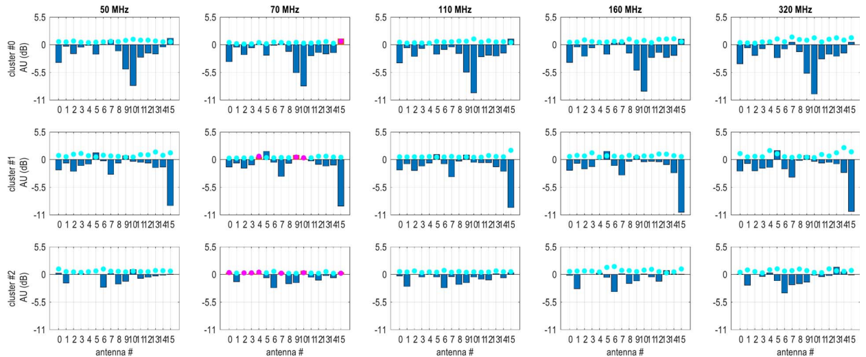
Figure 5. Synoptic visualization of the EDA2 results. Clusters from 0 to 2 in each row. Frequencies from 50 MHz to 320 MHz in each column. Dots: RMS discrepancy between measured and simulated EEP. Bars: measured relative active element gain.
