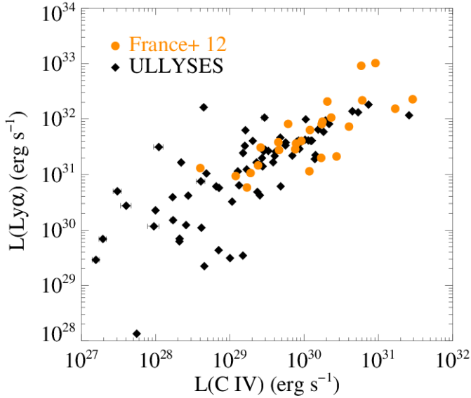
Figure 5. Comparison of the C IV and Ly \alpha luminosities of the ULLYSES stars (black diamonds) and previous HST -COS survey of CTTS ( France et al. 2012b ; orange circles). The plot demonstrates the correlation between Ly \alpha (as derived in Section 3.1) and accretion-dominated emission from C IV. This is consistent with the broad, bright Ly \alpha profiles of CTTS ( Schindhelm et al. 2012b ; Arulanantham et al. 2023 ) being powered by mass accretion (e.g., France et al. 2014b ).
