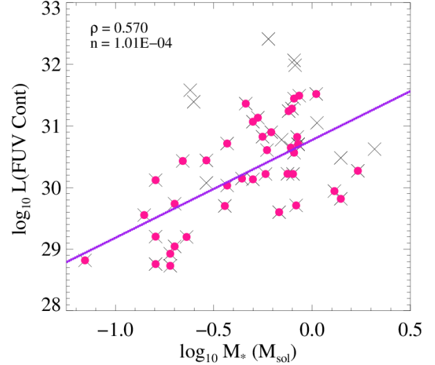
Figure 6. The FUV continuum luminosity increases with pre-main sequence stellar mass. The stars in the ULLYSES sample with good measurements of the average H_2 emitting radius are shown with a black x, and those with literature A_V < 1 are overlaid with pink circles (see Section 3.3 and 4.1). A fit to the A_V < 1 points is overplotted in purple. The Spearman rank coefficient ( \rho ) and probability coefficient for null correlation ( n ) of the A_V < 1 points are shown at the upper left.
