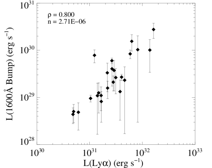
Figure 10. The 1600Å Bump luminosity is strongly correlated with Ly\alpha luminosity. This correlation supports the hypothesis that the Bump is powered by Ly\alpha -driven H_2O dissociation. The Spearman rank coefficient ( \rho ) and probability coefficient for null correlation ( n ) are shown at the upper left.
