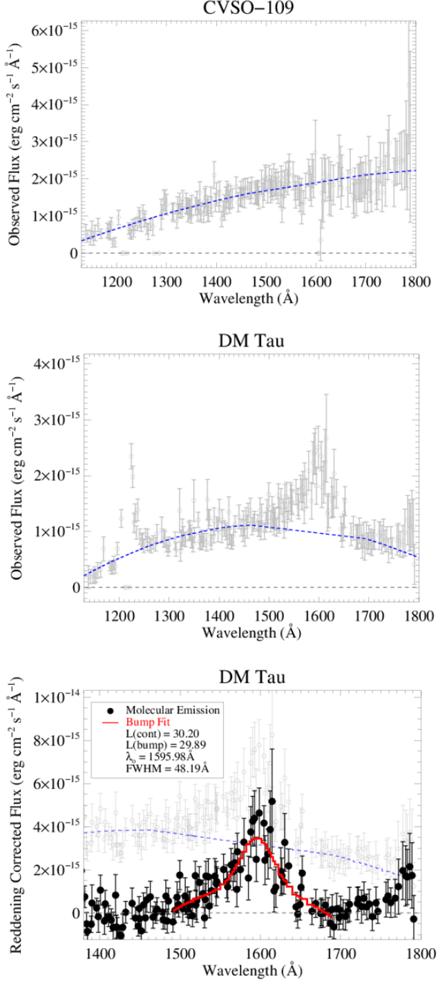
Figure 3. Example FUV continuum spectra for two targets in the ULLYSES DR5, CVSO 109 (top panel; Espaillet et al. 2022 ) and DM Tau (center panel). The underlying accretion continuum (fit with a polynomial; blue dashed line) is removed and the residual molecular continuum is shown as the black circle data points in the bottom panel. The molecular continuum fit is parameterized by a Gaussian + polynomial ( France et al. 2017 ) and is shown in red. Molecular continuum fit parameters are shown in the legend; the \log_{10} (luminosity) of the FUV continuum and the 1600 Å Bump, in units of \text{erg s}^{-1} , are presented as L(\text{cont}) and L(\text{bump}) , respectively
