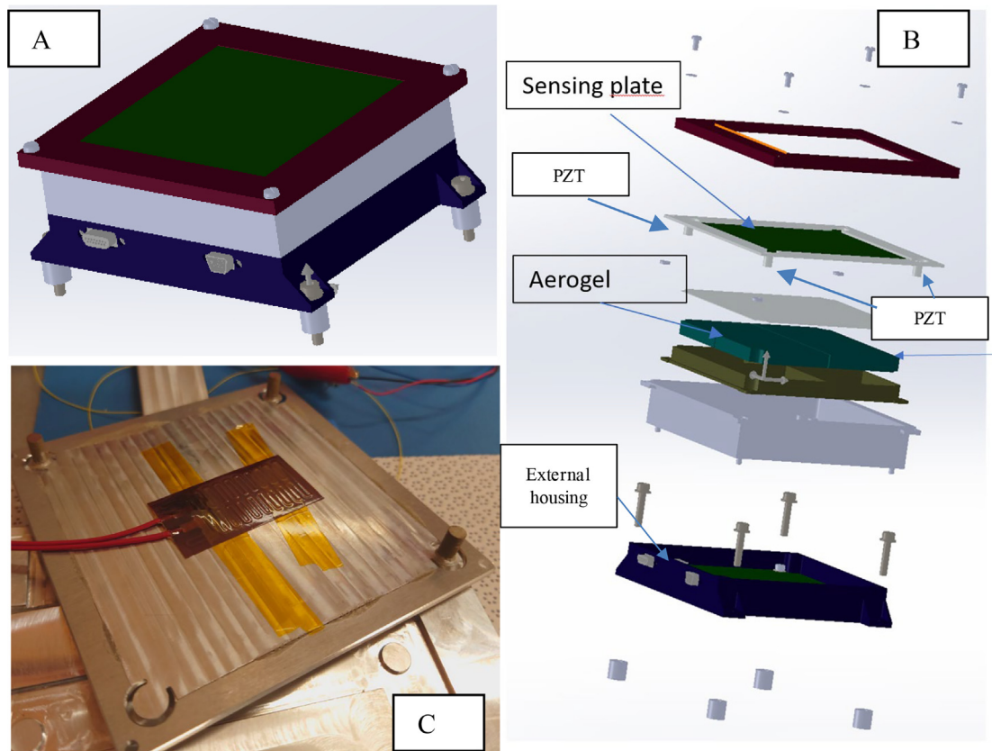
Fig. 1. A) DISC instrument 3D CAD model; B) DISC exploded view: sensing plate equipped with piezoelectric transducers, aerogel dust shield, electronic boards, external housing; C) DISC sensing plate with 3 PZT glued at the corners.
