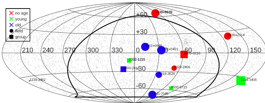
Figure 10. An Aitoff projection displaying the sky positions for the 14 CYSs within 50 pc. Note that 0339+6639 comprises two stars in a resolved binary system. The colour scheme provides an age estimate for the stars based on assessment of Li EW, where objects in red lack any Li EW measurement therefore have an indeterminate age, blue symbols are objects that have no indication of youth, and green symbols are likely to be at least as young as the Pleiades. Square symbols indicate objects that belong to the potential MG member list in Table 6, even if they are suggested to be non-members in Section 5.1. Circles represent stars that have no entry in Table 6 and are very likely to be nearby field stars. The relative sizes of the symbols represent distance, with the closest stars appearing the largest. The small black dots on the plot represent \sim 6000 K-stars within 50 pc identified in DR1 and the enclosed solid-black loop is the Galactic Plane.
