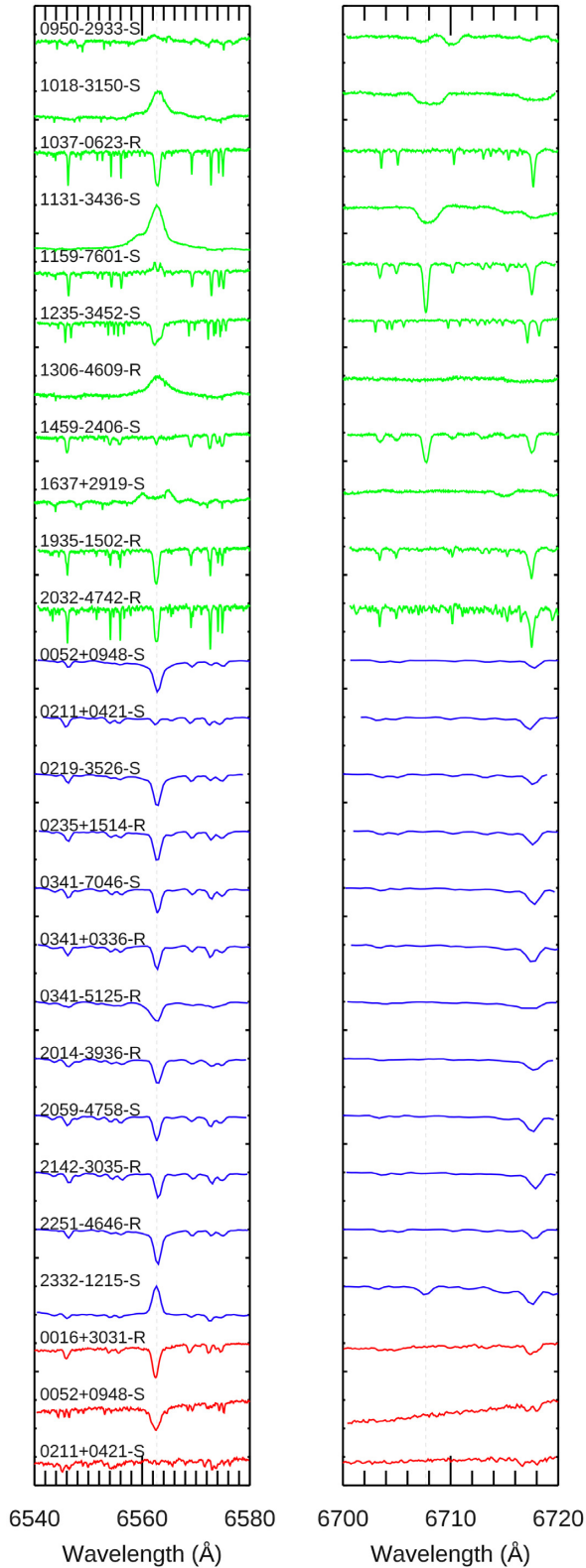
Figure 3. Spectra for the candidates observed at the SPM (red), ANU (blue), and MIKE (green) around the H\alpha feature at 6563 Å (left) and the Li I feature at 6708 Å (right). The name suffixes ‘S’ and ‘R’ indicate whether the star survives or is rejected from the CYS sample based on the DR2 astrometric criteria.
