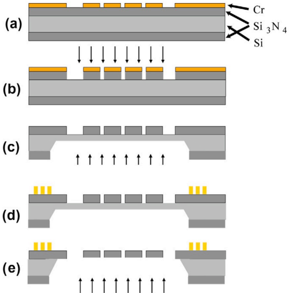
Figure 3. Schematic view of the fabrication process as described in the text. The Process starts with a commercial 3 inch silicon wafer <100> oriented and covered on both sides with a 1 \mu\text{m} thick low stress silicon nitride layer as described in the text.
