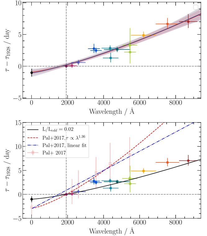
Figure 4. Inter-band lag spectrum of Fairall 9. Top panel: CCF lags as a function of wavelength for the Swift and LCO bands. All lags are measured with respect to the Swift /UVW2 band. The best-fitting relation for the reprocessing model ( \tau \propto \lambda^{4/3} ) is shown as the red line and its 1\sigma error envelope is the shaded region. The black solid line and error envelope shows the fit when leaving the power-law index as a free parameter. Bottom panel: lag spectrum comparison between this work and the inter-band lags measured by Pal et al. (2017). We show their linear (blue) and exponential fits (red). The predicted lag spectrum for Fairall 9 is shown as the black line. This shows the clear need of IDRM campaigns to extract the lag spectrum with high accuracy.
