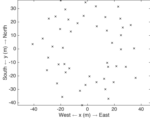
Fig. 1: Nominal antenna positions.
