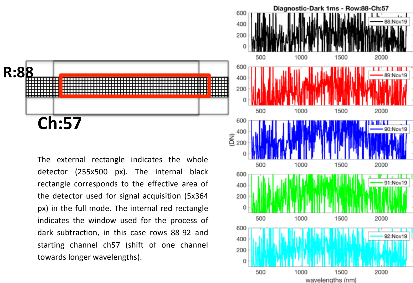
Fig.27. Diagnostic (OP31, Ses#2, Nov'19) after dark subtraction on rows 88-92. The dark#2 from OP30 was used. On the left the window used for dark subtraction, corresponding to nominal rows 88-92 and starting channel 57.
