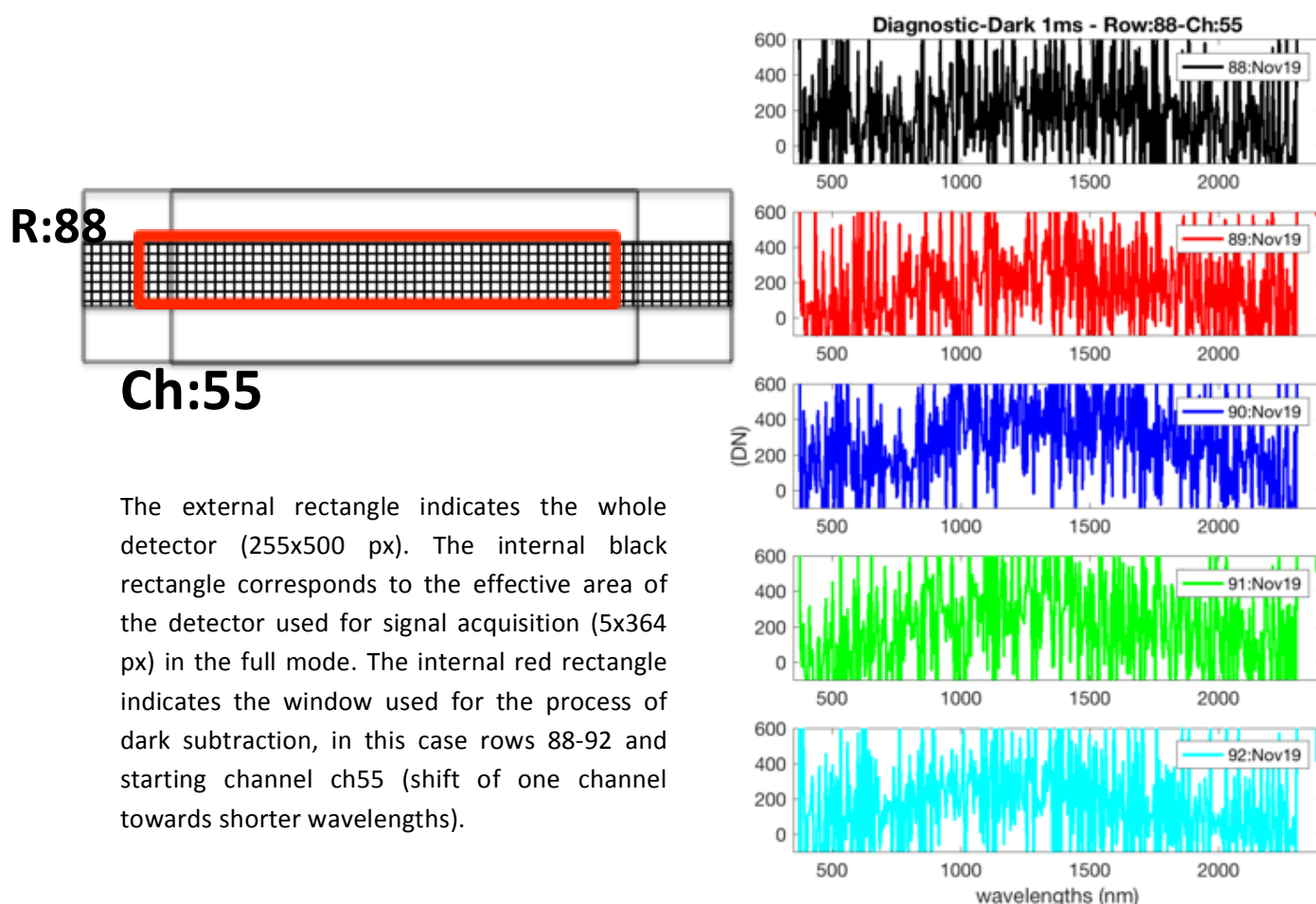
Fig.28. Diagnostic (OP31, Ses#2, Nov'19) after dark subtraction on rows 88-92. The dark#2 from OP30 was used. On the left the window used for dark subtraction, corresponding to nominal rows 88-92 and starting channel 55.
