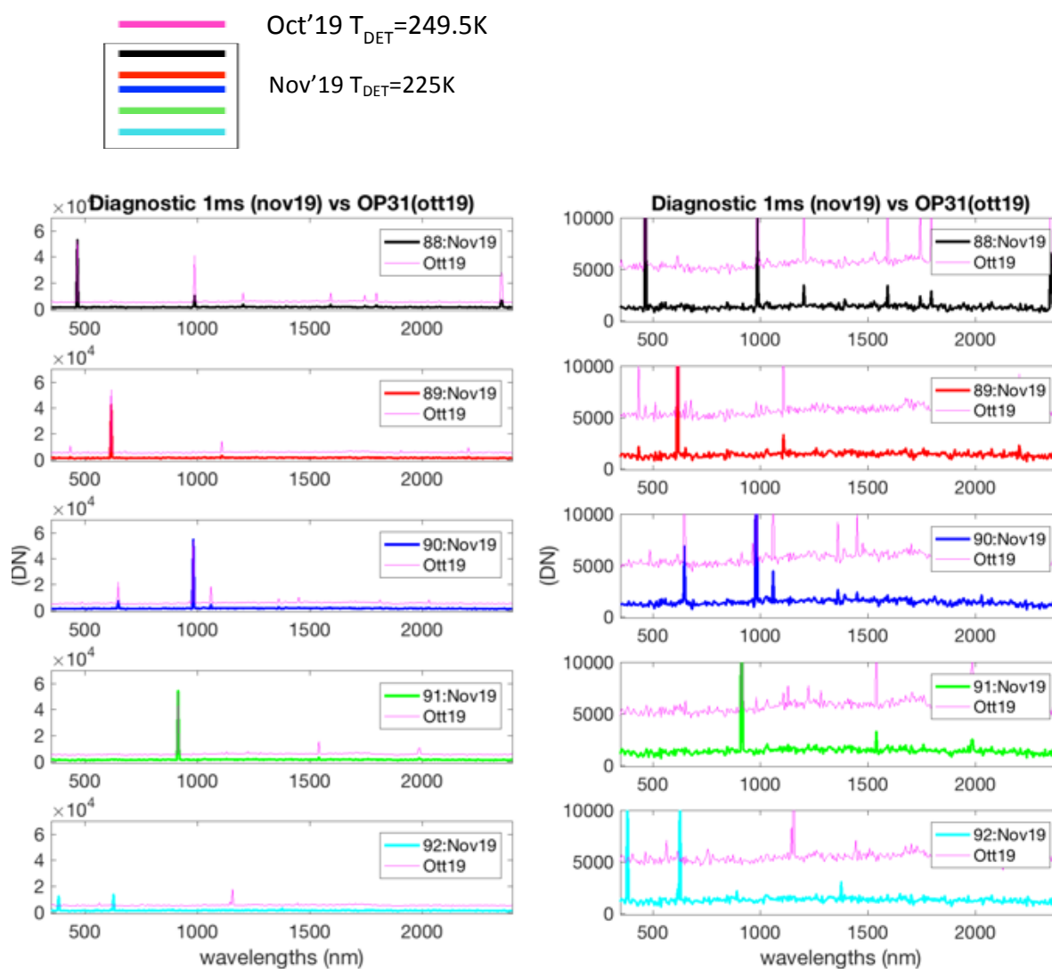
Fig.25. The OP31 acquired in Nov'19 (Session#2, cold) compared with the OP31 acquired in Oct'19 (Session#1, hot). On the right the view is zoomed along the Y-axis.
