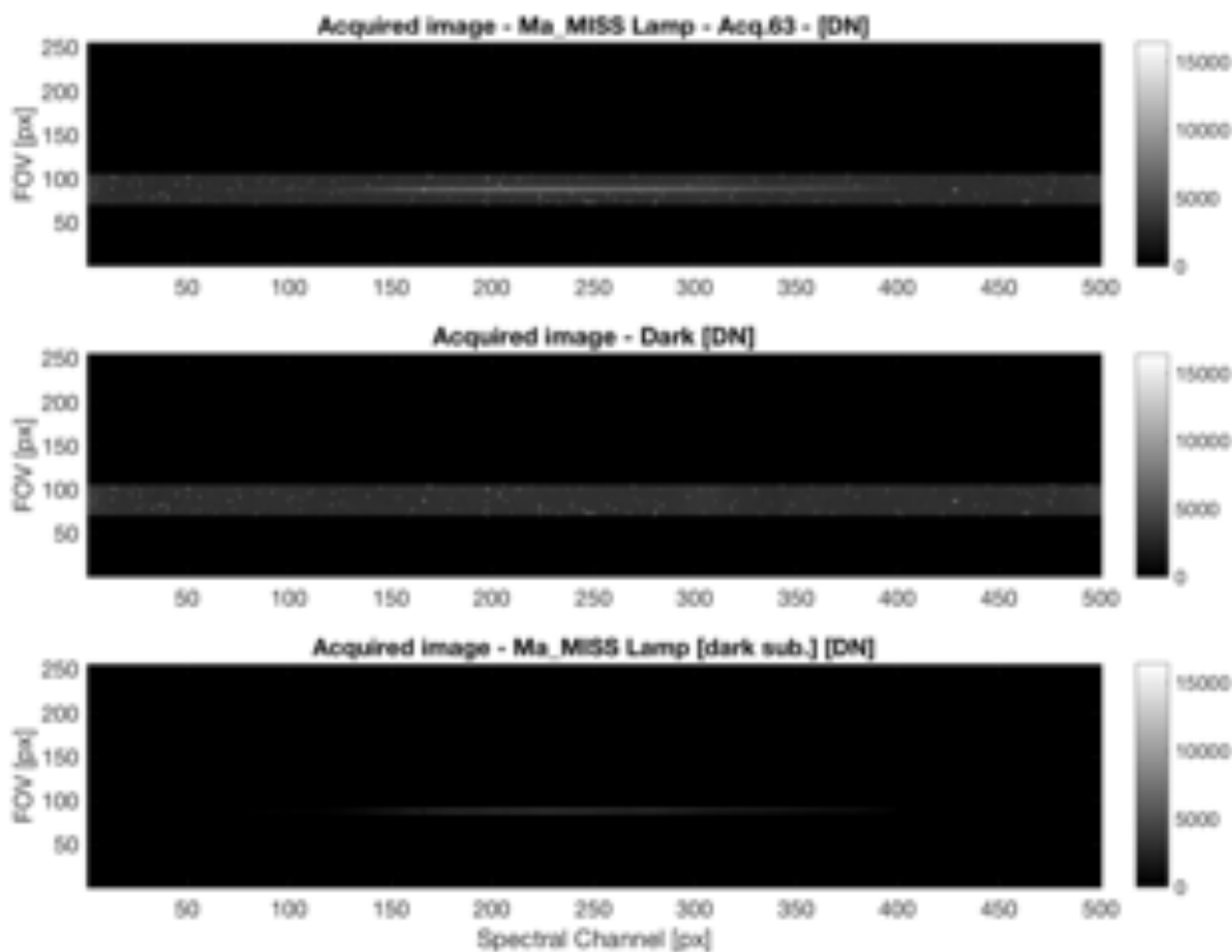
Fig.9. Diagnostic acquired during spectrometer alignment phase (2017)
