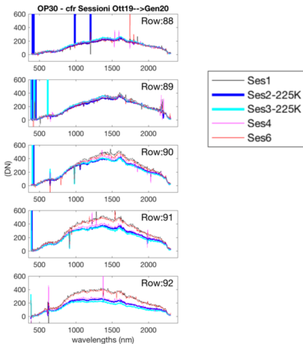
Fig.44. OP30 after dark correction; comparison between different sessions.
