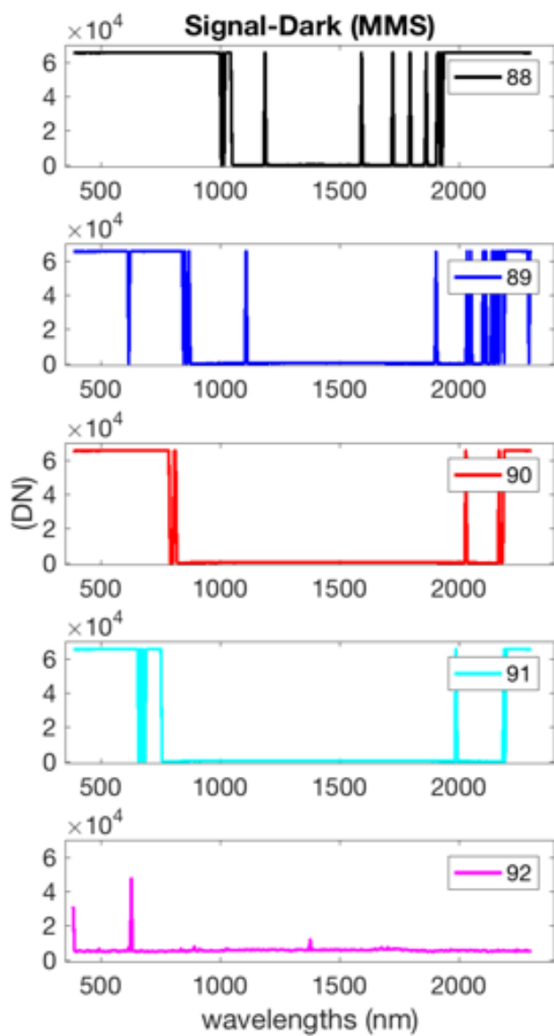
Fig.4. OP30, signal with dark automatically subtracted by Ma_MISSION SW
