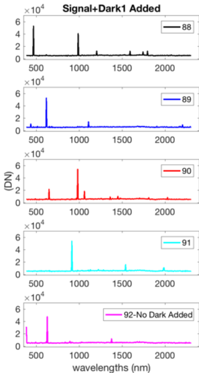
Fig.5. OP30: the signal in fig.3, after manual addition of dark 1
