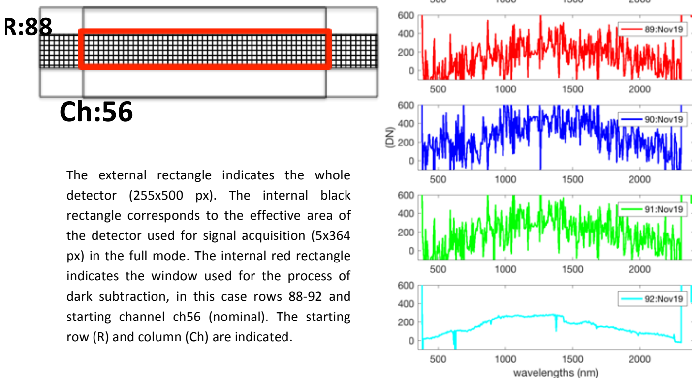
Fig.26. Diagnostic (OP31, Ses#2, Nov’19) after dark subtraction on rows 88-92. The dark#2 from OP30 was used. On the left the window used for dark subtraction, corresponding to nominal rows 88-92 and starting channel 56.
