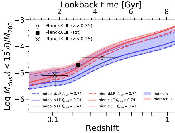
Figure 2. The black points represent the average Planck dust mass measured within 15 arcmin of a stacked cluster sample (PlanckXLIII-16). All three masses are normalized to the average M_{200} of their respective bins. The full square is the full sample ( M_{200} \simeq 5.6 \times 10^{14} M_{\odot} and z \sim 0.26 ). The ‘x’ is the nearby ( z < 0.25 ) bin of average mass M_{200} \simeq 4.3 \times 10^{14} M_{\odot} , the hollow diamond is the distant ( z > 0.25 ) bin ( M_{200} \simeq 7.0 \times 10^{14} M_{\odot} ). The curves follow the integrated dust evolution computed in this work, as they would be seen within a fixed aperture of 15 arcmin from the cluster centre, normalized by M_{200} . We perform this rescaling to mimic the Planck data. The blue curves identify the case in which the morphologies evolve independently, whereas the red curves show the case in which morphologies merge in accordance to hierarchical clustering. The solid curves assume a single LF, and the dashed curve a double LF, calibrated on the WINGS cluster survey (Moretti et al. 2015). The thick curves assume an elliptical fraction of f_{0,ell} = 0.74 , as in the WINGS clusters. The fainter curves assume instead a f_{0,ell} = 0.43 . This is the fraction of the Virgo cluster and it is representative of other similarly young and active clusters. The semitransparent red and blue bands span – for the independent and hierarchical evolution – an f_{0,ell} between 0.2 and 0.82, the latter being the elliptical fraction of the Coma cluster, representative of fully evolved clusters.
