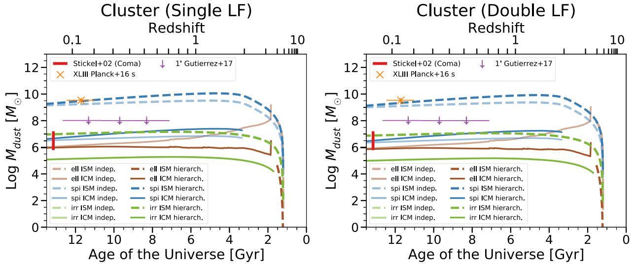
Figure 1. The evolution of dust mass components within a WINGS-like average cluster ( M_{200} \sim 5 \times 10^{14} M_{\odot} , f_{\text{ell}} = 0.74 , n^* = 52 ). The brown, blue, and green lines represent elliptical/S0, spiral, and dwarf irregular galaxies, respectively. The dashed lines identify the integrated dust component residing within galaxies (ISM), whereas the solid lines identify the ejected components (ICM). The semitransparent lines are computed assuming that each morphology evolves independently, whereas the fully opaque lines are computed assuming a hierarchical clustering scenario. All morphologies begin their evolution 1.2 Gyr after the big bang (or at redshift z \sim 5 ). The orange ‘x’ is the Planck XLIII-16 subsample at low redshift, whose average cluster mass is M_{200} = 4.3 \times 10^{14} M_{\odot} . The purple downward arrows are the upper limits found in GLC17 for the 350 \mu\text{m} Herschel beam within a radius of 1 arcmin. The three redshift bins are centred around redshift z = 0.173, 0.338 , and 0.517 ; they include clusters with total masses > 10^{14} M_{\odot} . In red is the dust estimate from Stickel et al. (2002) for the Coma cluster.
