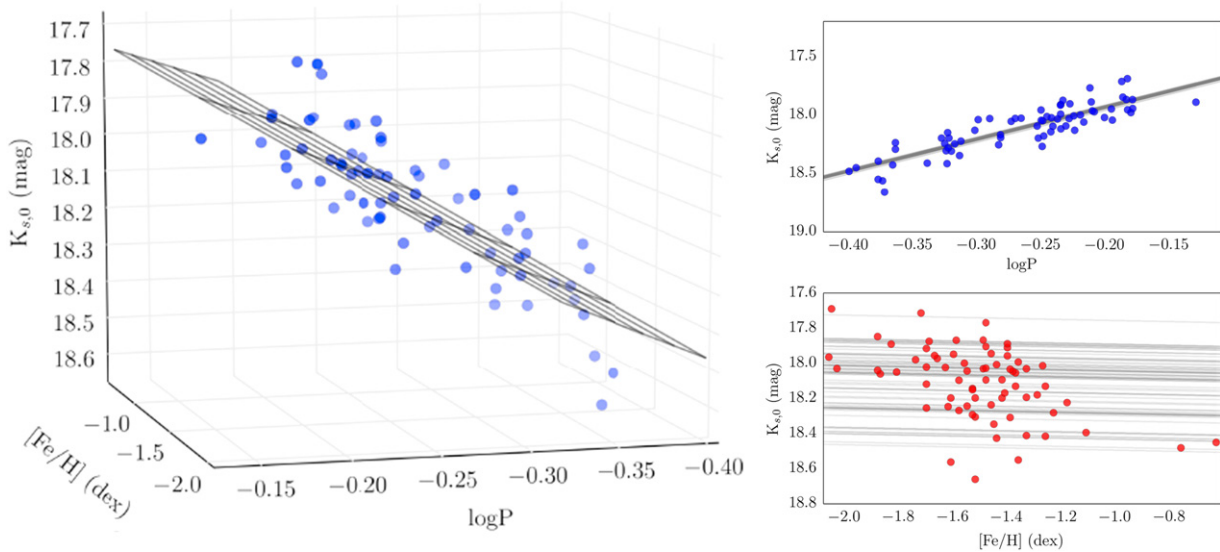
Figure 2. Left panel: PL K s Z relation of the 70 LMC RR Lyrae stars (Equation (3)) analyzed in the paper, in the period–luminosity–metallicity space. Right panels: projections of the PL K s Z relation (Equation (3)) on the \log(P) - K_s (top) and K_s - [\text{Fe}/\text{H}] (bottom) planes. Gray lines represent lines of equal metallicity (top) and equal period (bottom). See the text for the details. Uncertainties in the K_s magnitude and [\text{Fe}/\text{H}] are omitted to simplify the figure, but they are provided in Table 1.
