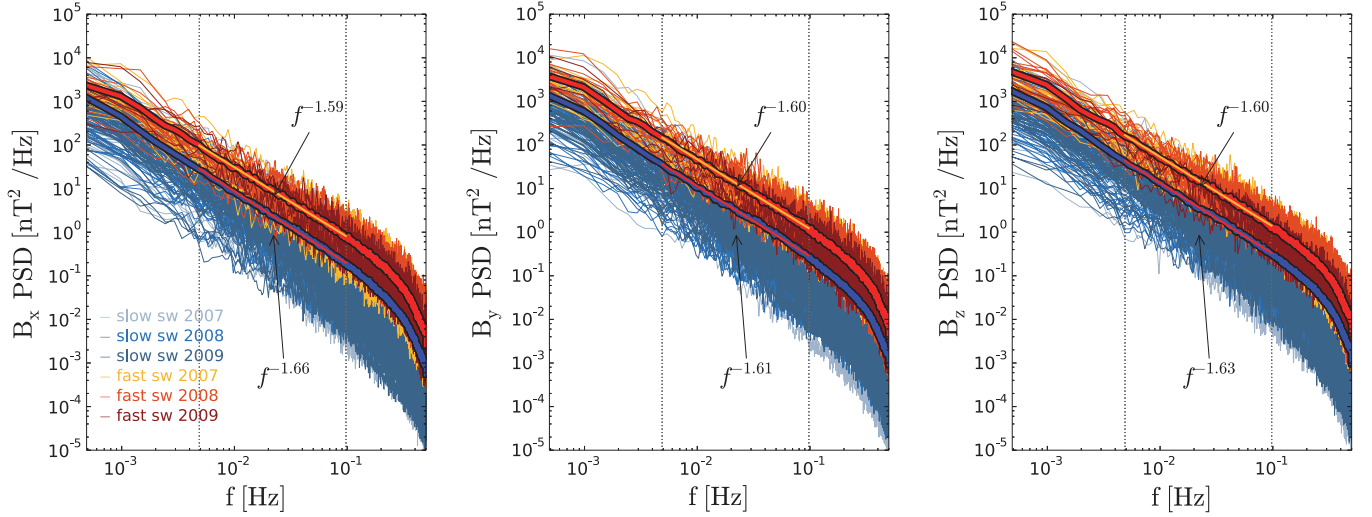
Figure 1. Summary plot of the power spectral density spectrum of B_x , B_y , and B_z from VEX magnetic field data recorded between 2007 and 2009, during the minimum of the 24th solar cycle. Yellow and red lines correspond to fast solar wind, gray and blue lines correspond to slow solar wind. The black dotted lines mark the frequency interval for which the spectral index of each spectrum is computed. An average spectrum is derived as an ensemble average of all the spectra obtained for the fast (the embossed red line) and slow wind (the embossed blue line), respectively. The spectral slope of the average spectra is computed for the frequency range marked by yellow and magenta, respectively.
