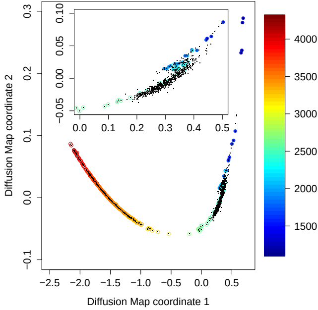
Fig. A.1. Projection onto the first two diffusion map coordinates of the set of 995 spectra defined in Sect. A.3. The colour code reflects the temperatures assigned according to their spectral types (filled circles) or literature values (empty circles). Black dots represent the entire set of sources used to construct the diffusion map. The inset plot is a zoom of the problematic zone around 2000 K where temperature variations causes only very subtle changes in the RP spectrum.
