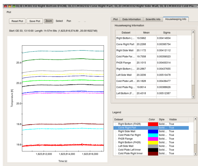
Figure 2 – Front-end temperature during CRYO-02 test in CSL (left) and during CPV (right)
