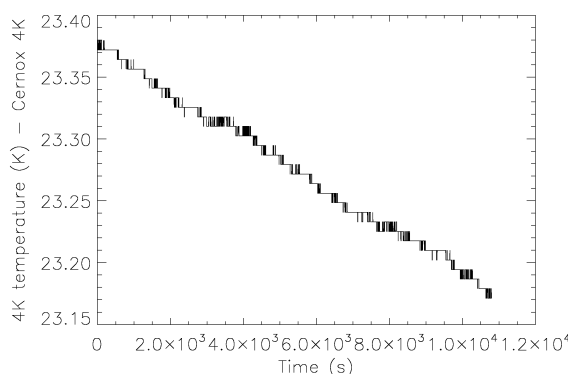
Figure 1 – Reference load temperature during CRYO-02 test in CSL (left) and during CPV (right)
