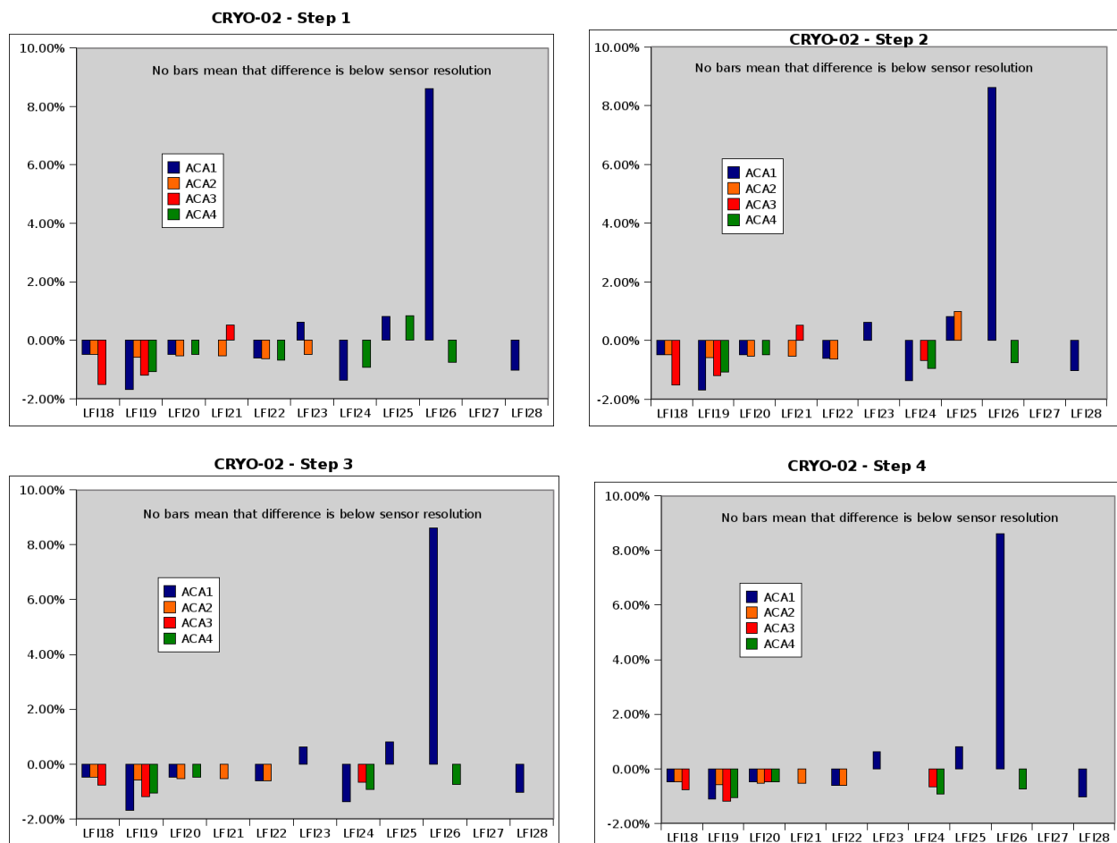
Fig. 6 – Comparison of drain currents measured during CRYO-02 test in CPV and in CSL. The percentage variation is defined by (I_d(\text{CPV}) - I_d(\text{CSL}))/I_d(\text{CSL}) . Where no bars are displayed it means that the drain current variation was less than 0.1 mA
