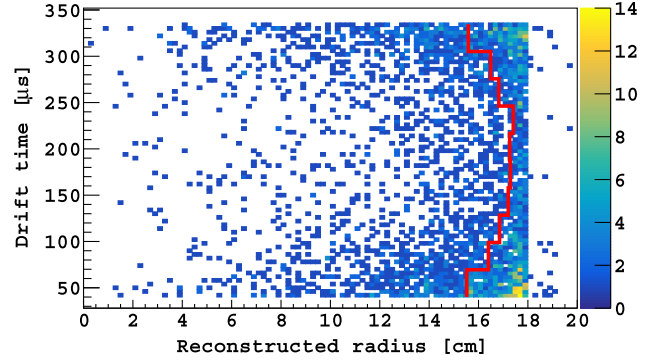
FIG. 5. Radial cut (red) shown on events in the initial blinding box shown in Fig. 4. All event quality cuts (Sec. VIA 1), all basic cuts (Sec. VIA 2) through MinS2uncorr , and vertical fiducialization via t_{\text{drift}} have been applied.
