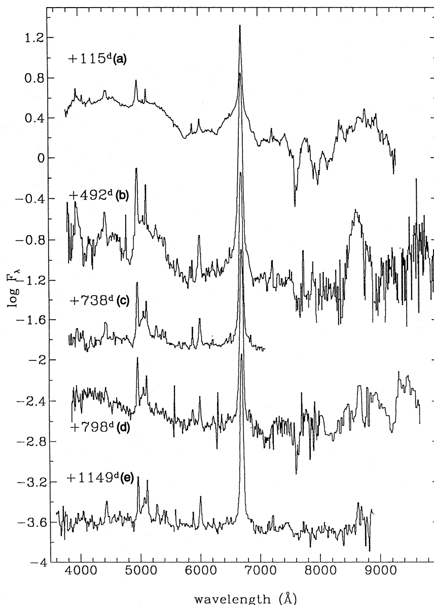
Figure 5. The spectral evolution of SN 1988Z on the EFOSC1 spectra (cf. Table 2). The ordinate scale is \log F_\lambda , where fluxes are in 10^{-16}\text{ erg s}^{-1}\text{ cm}^{-2}\text{ \AA}^{-1} , and the observed wavelength is on the abscissa. Spectra (b), (c), (d) and (e) have been down-shifted by 0.7, 1.3, 2.1 and 2.8, respectively.
