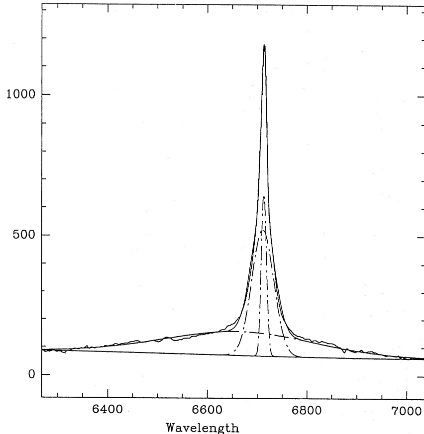
Figure 7. The deconvolution into three components of the profile of H\alpha at phase 115 d. The parameters of the three components are given in Table 5. The dot-dashed lines represent the single components, while the solid lines represent the global fit and the observed profile.
