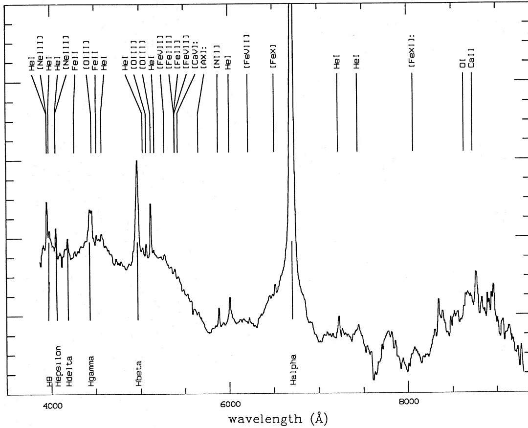
Figure 6. Line identifications on the spectrum at day 115.
