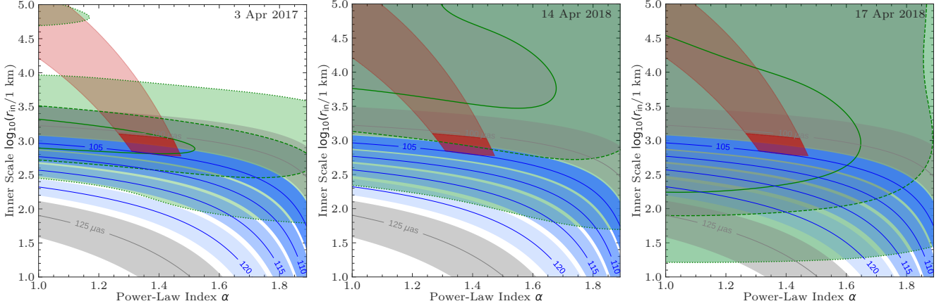
Figure 8. Same as Figure 7, but with the added THEMIS posterior distributions from simultaneous intrinsic source and scattering parameter fitting overlaid in green. The 1\sigma , 2\sigma , and 3\sigma regions are shown from dark green to light green. The solid, dashed, and dotted lines are the 1\sigma , 2\sigma , and 3\sigma contours respectively.
