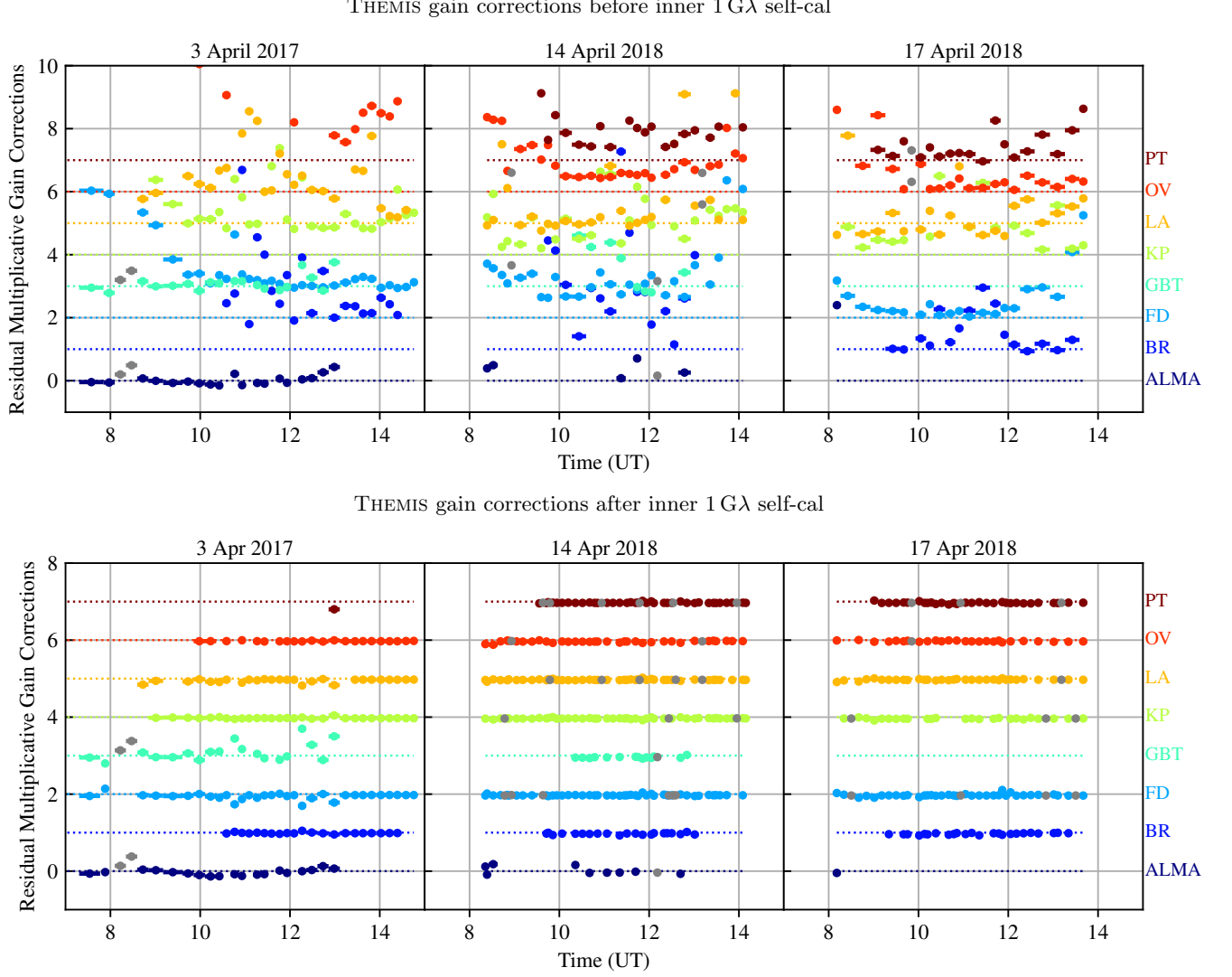
Figure 9. Residual multiplicative gain corrections derived by THEMIS in the Sgr A* model fitting for all three observing days. Top: Residual variations in the amplitudes derived from the data sets where only a priori amplitude corrections are applied. Bottom: Residual variations in the amplitudes derived from the data sets already corrected based on self-calibration (see Section 3.2). For 3 April 2017, inner 1 G \lambda self-cal gain corrections were not applied to the GBT due to the scatter introduced by its baseline to NL, whose measurements dominate within that baseline cut (Issaoun et al. 2019b). In all panels, individual station gain corrections are offset vertically by unity for clarity, with the dashed horizontal lines indicating a unit gain for each station. The gain correction scale is linear. Each point corresponds to an individual scan: colored points are independently reconstructed in the procedure, grey points are not well constrained due to missing information and are thus heavily biased by the prior.
