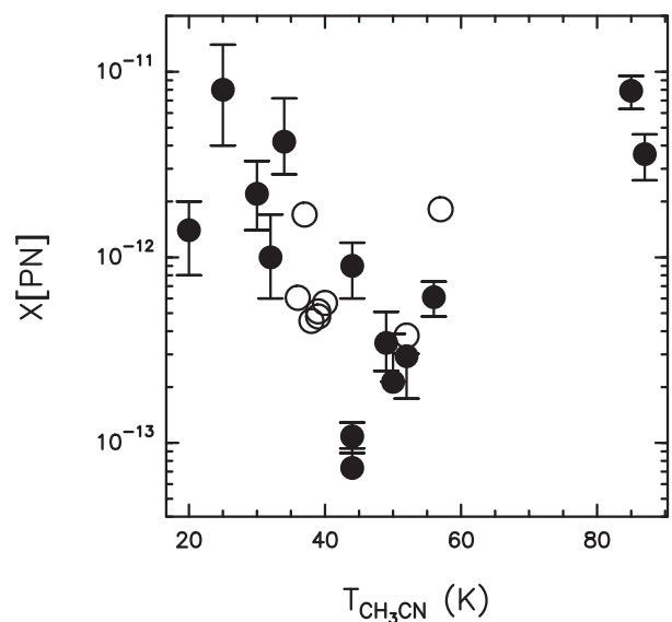
Figure 10. PN abundance against gas temperature estimated from CH_3CN (Colzi et al. 2018). Empty symbols correspond to X[PN] upper limits.
