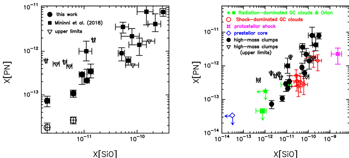
Figure 9. Left: Comparison between the abundances relative to H_2 of PN and SiO, X[PN] and X[SiO] , respectively. Circles and squares indicate the results obtained in this work and by Mininni et al. (2018), respectively. Only the sources in which SiO, PN, and H_2 column densities could have been derived, or having upper limits on N(PN) , are shown. For G037.55+0.19 and G048.99–0.30, the PN column density has been estimated assuming 4 and 16 K, hence the abundance has two estimates as well: the open circles indicate X[PN] when T_{ex} = 4 K, and the filled points having the same X[SiO] of the empty ones correspond to X[PN] when T_{ex} = 16 K. The open triangles indicate the N(PN) upper limits. Right: X[PN] against X[SiO] for the high-mass star-forming clumps illustrated in the left-hand panel (filled circles) compared to the measurements of Rivilla et al. (2018) in other regions located in different places of the Galaxy: shock-dominated Galactic Centre clouds (red circles) and radiation-dominated Galactic Centre clouds (green stars), the Orion Bar (green square; Cuadrado, private communication), the L1157-B1 shock (magenta open star, Lefloch et al. 2016), and the L1544 pre-stellar core (blue open diamond; from the data set from Jiménez-Serra et al. 2016). The plot is the updated version of fig. 3 of Rivilla et al. (2018).
