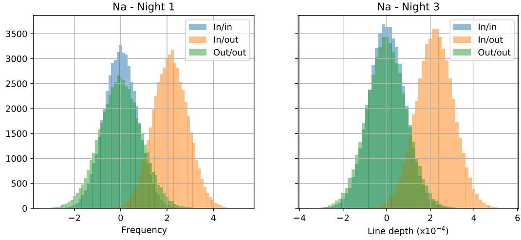
Supplementary Data Figure 2: The distributions of randomly generated instances of the one-dimensional cross-correlation function at the rest-frame velocity of the planet for the Na doublet, for each of the two nights in which the transit was fully covered. The in- and out-of-transit master functions are constructed by taking random subsets of the in-, resp. out-of-transit exposures. The measured line depth is expected to be around zero for out-out (in green) and in-in (in blue), i.e. where the randomly picked subset is normalised (subtracted) with its own master-spectrum. Only when the in-transit cross-correlation functions are normalised by the out-of-transit master spectrum (in-out, in orange), we expect the measured line amplitude to be different from zero.
