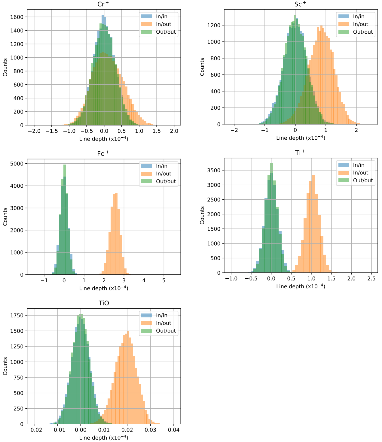
Supplementary Data Figure 10: The distributions of randomly generated instances of the one-dimensional cross-correlation function for Cr + , Fe + , TiO, Sc + and Ti + at the rest-frame velocity of the planet. The in- and out-of-transit master functions are constructed by taking random subsets of the in-, resp. out-of-transit exposures. The measured line depth is expected to be around zero for out-out (in green) and in-in (in blue), i.e. where the randomly picked subset is normalised (subtracted) with its own master-spectrum. Only when the in-transit cross-correlation functions are normalised by the out-of-transit master spectrum (in-out, in orange), we expect the measured line amplitude to be different from zero. Al seemingly presents a detection using this bootstrap method, but comparing to Supplementary Fig. 12 shows that there is no signal present in the K_p - V_{\text{sys}} diagram
