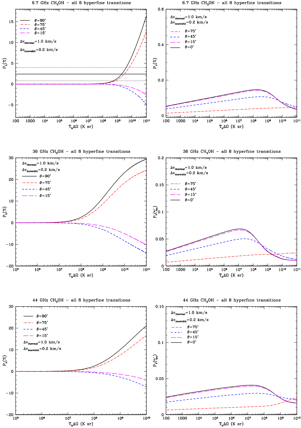
Figure 1. Outputs of the FRTM code for the 6.7 GHz, 36 GHz, and 44 GHz \text{CH}_3\text{OH} maser emissions. The plots are obtained by assuming that all the eight hyperfine transitions, which are listed in Lankhaar et al. (2017), contribute equally to the maser emission. Left panels: the fractional linear polarization vs. the emerging brightness temperature. The horizontal black dashed lines indicate the range of typical P_L measured towards 6.7 GHz \text{CH}_3\text{OH} masers. Right panels: the fractional circular polarization vs. the emerging brightness temperature.
