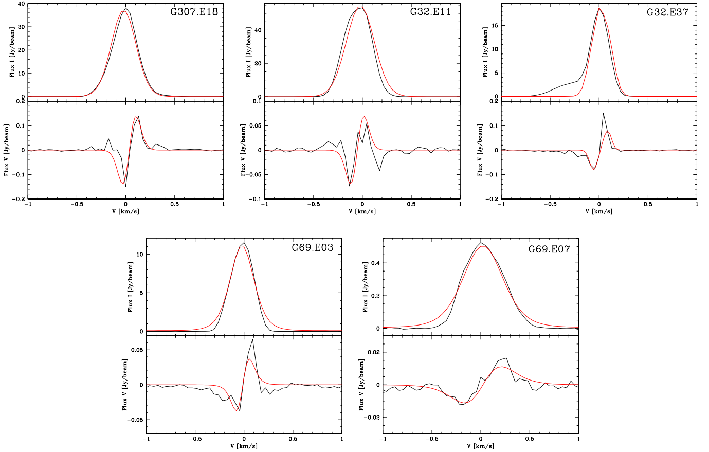
Fig. 2. Total intensity ( I , upper panel) and circularly polarized intensity ( V , lower panel) spectra for the CH 3 OH maser features called G307.E18, G32.E11, G32.E37, G69.E03, and G69.E07 (see Tables A.1, A.4, and A.5). The thick red lines are the best-fit models of I and V emissions obtained using the adapted FRTM code (see Sect. 3). The maser features were centered on zero velocity.
