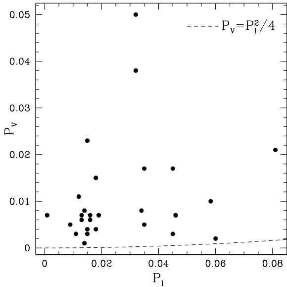
Fig. 11. Circular polarization fraction ( P_V ) of the 6.7 GHz \text{CH}_3\text{OH} maser features as function of the corresponding linear polarization fraction ( P_1 ). The dashed line represents the conversion of P_1 into P_V due to the rotation of 1 rad in the magnetic field along the maser path (Dall’Olio et al. 2020). The data are taken from: Surcis et al. (2009, 2011a, 2014b), Vlemmings et al. (2010), Papers I–IV, and this work.
