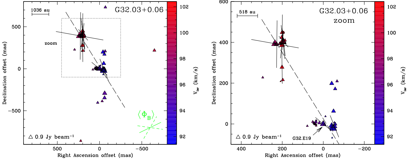
Fig. 5. View of the CH 3 OH maser features detected around G32.03+0.06 (Table A.4) (left panel). The symbols are the same as in Fig. 1. The polarization fraction is in the range P_l = 0.4 - 10.0\% (Table A.4). The assumed velocity of the YSO is V_{\text{lsr}}^{\text{CO}} = +96.3 \text{ km s}^{-1} (Areal et al. 2018). The dashed line is the best least-squares linear fit of the CH 3 OH maser features ( \text{PA}_{\text{CH}_3\text{OH}} = +32^\circ \pm 7^\circ ). Right panel: zoom-in view.
