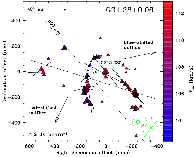
Fig. 4. View of the CH 3 OH maser features detected around G31.28+0.06 (Table A.3). The symbols are the same as in Fig. 1. The polarization fraction is in the range P_1 = 0.5 –16.7% (Table A.3). The assumed velocity of the YSO is V_{\text{lsr}}^{\text{CO}} = +108.3 km s -1 (Yang et al. 2018). The dashed line is the best least-squares linear fit of the CH 3 OH maser features ( \text{PA}_{\text{CH}_3\text{OH}} = +73^\circ \pm 4^\circ ). The two arrows indicate the direction and not the actual position of the red- and blueshifted lobe of the outflow ( \text{PA}_{\text{CH}_3\text{OH}}^{\text{outflow,blue}} = -78^\circ and \text{PA}_{\text{CH}_3\text{OH}}^{\text{outflow,red}} = +154^\circ , Yang et al. 2018). The dotted line indicates the orientation of the 850 \mu\text{m} emission detected by Thompson et al. (2006).
