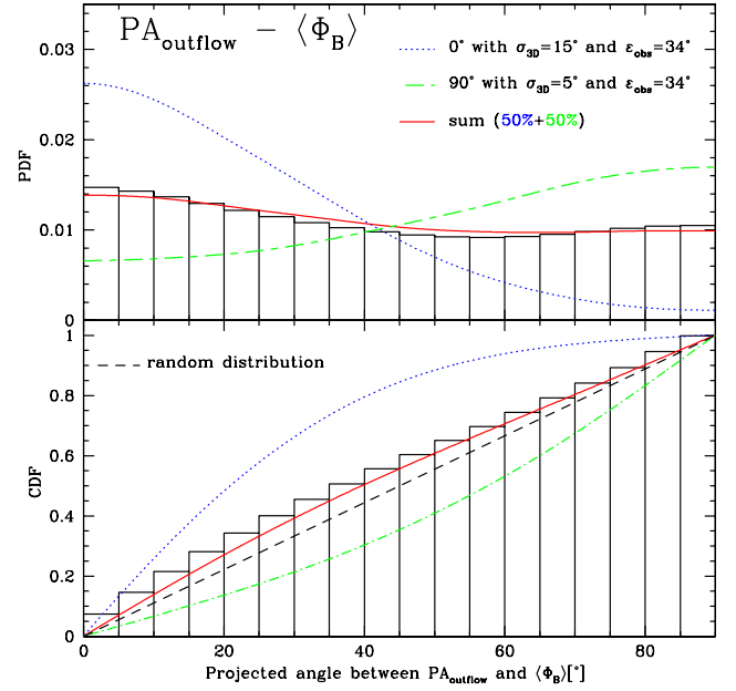
Fig. 7. Probability distribution function ( top panel ) and the cumulative distribution function ( bottom panel ) of the projected angle between the magnetic field and the outflow axes ( |\text{PA}_{\text{outflow}} - \langle\Phi_B\rangle| ). The dotted blue line is the result of a Monte Carlo simulation of the projection on the plane of the sky of two random 3D parallel vectors with a Gaussian uncertainty of 15° and with a projected Gaussian error of 34° (called 0 deg distribution). The dot-dashed green line is the result of a Monte Carlo simulation of the projection on the plane of the sky of two random 3D perpendicular vectors with a Gaussian uncertainty of 5° and with a projected error of 34° (called 90 deg distribution). The red line is the best combination of the previous two simulations to fit the observed data. Here, both the 0 deg distribution and the 90 deg distribution contribute to the 50%. The dashed black line is the CDF for a completely random orientation of outflows and magnetic fields, i.e., all angular differences are equally likely. The results of the K–S test are listed in Table 3.
