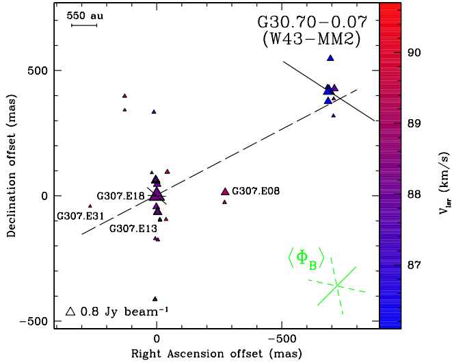
Fig. 1. View of the CH 3 OH maser features detected around G30.70-0.07 (W43-MM2). The reference position is the estimated absolute position from Table 1. Triangles identify CH 3 OH maser features whose side length is scaled logarithmically according to their peak flux densities (Table A.1). Maser local standard of rest radial velocities are indicated by color (the assumed velocity of the region is V_{\text{lsr}}^{\text{SiO}(2-1)} = +91.0 \text{ km s}^{-1} ; Nguyen-Lu’o’ng et al. 2013). The 0.8 \text{ Jy beam}^{-1} symbol is plotted for comparison. The linear polarization vectors, scaled logarithmically according to the polarization fraction P_1 ( P_1 = 0.07\text{--}1.2\% ; see Table A.1), are overplotted. In the bottom right corner, the corresponding error-weighted orientation of the magnetic field ( \langle \Phi_B \rangle , see Sect. 5.1) is also shown. The two dashed segments indicate the uncertainty. The dashed line is the best least-squares linear fit of the CH 3 OH maser features ( \text{PA}_{\text{CH}_3\text{OH}} = -67^\circ \pm 7^\circ ).
