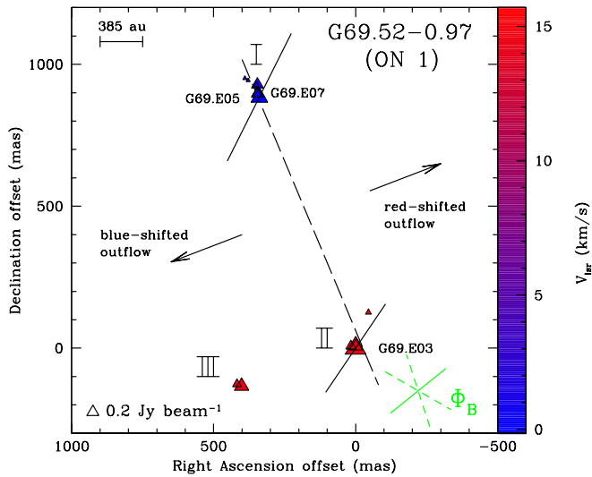
Fig. 6. View of the CH 3 OH maser features detected around G69.52-0.97 (Table A.4). Same symbols as in Fig. 1. The polarization fraction is in the range P_l = 1.3-1.5\% (Table A.5). The assumed velocity of the YSO is V_{\text{lsr}}^{\text{CS}} = +11.6 \text{ km s}^{-1} (Bronfman et al. 1996). The dashed line is the best least-squares linear fit of the CH 3 OH maser features ( \text{PA}_{\text{CH}_3\text{OH}} = +23^\circ \pm 7^\circ ). The two arrows indicate the direction and not the actual position of the red- and blueshifted lobes of the outflow ( \text{PA}_{\text{outflow}}^{\text{CO}} = -69^\circ , Kumar et al. 2004).
