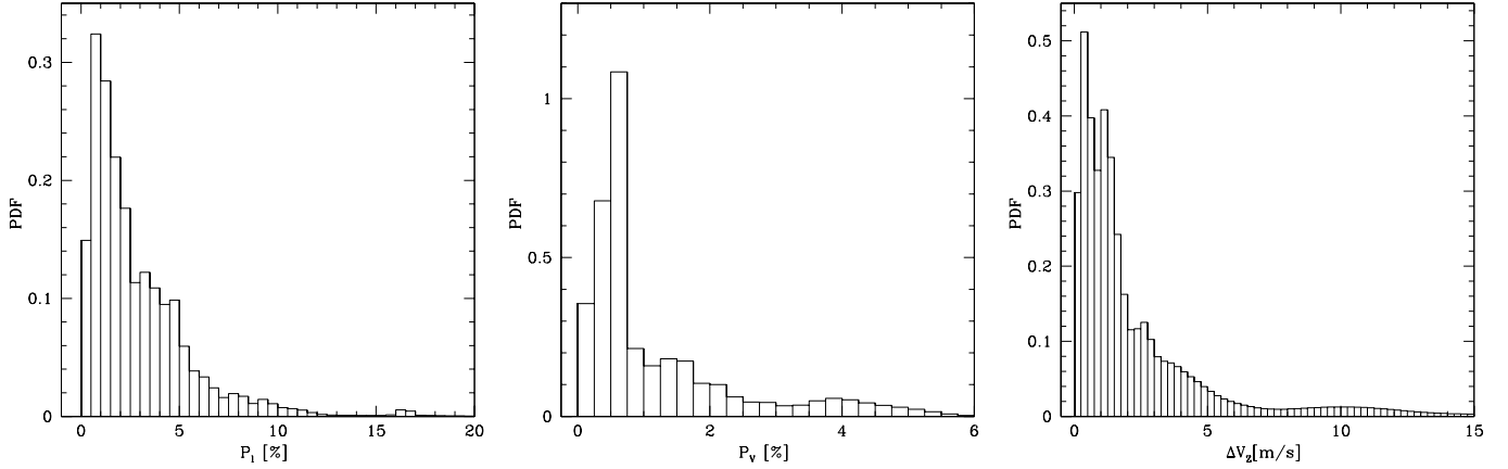
Fig. 9. Probability density function of the linear polarization fraction ( P_l , left panel ), of the circular polarization fraction ( P_v , middle panel ), and of the Zeeman-splitting ( \Delta V_Z , right panel ) of the 6.7 GHz \text{CH}_3\text{OH} maser emission. The interval width of the histograms is 0.5% and 0.25% and 0.25 \text{m s}^{-1} for the P_l , P_v , and the \Delta V_Z plots, respectively. The data are taken from: Surcis et al. (2009, 2011a, 2014b), Vlemmings et al. (2010), Papers I–IV, and this work.
