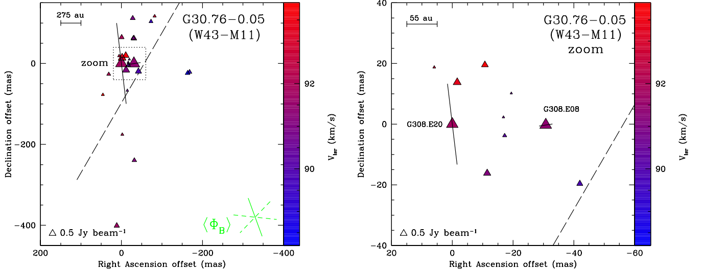
Fig. 3. View of the CH 3 OH maser features detected around G30.76-0.05 (Table A.2) (left panel). The symbols are the same as in Fig. 1. The polarization fraction is in the range P_1 = 0.4\text{--}1.9\% (Table A.2). The assumed velocity of the YSO is V_{\text{lsr}}^{\text{SiO}(2-1)} = +94.5 \text{ km s}^{-1} (Nguyen-Lu'o'ng et al. 2013). The dashed line is the best least-squares linear fit of the CH 3 OH maser features ( \text{PA}_{\text{CH}_3\text{OH}} = -30^\circ \pm 48^\circ ). Right panel: zoom-in view.
