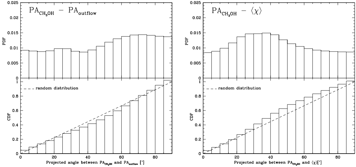
Fig. 8. Probability density function and CDF of the projected angle between the PA of the CH 3 OH maser distribution and the outflow axis ( |PA_{CH_3OH} - PA_{outflow}| ) (left). Right: Probability distribution function (top panel) and CDF (bottom panel) of the projected angle between the PA of the CH 3 OH maser distribution and the linear polarization angles ( |PA_{CH_3OH} - \langle\chi\rangle| ). In both panels the dashed line is the CDF for random distribution of the corresponding angles, i.e., all angular differences are equally likely. The results of the K–S test are listed in Table 3.
