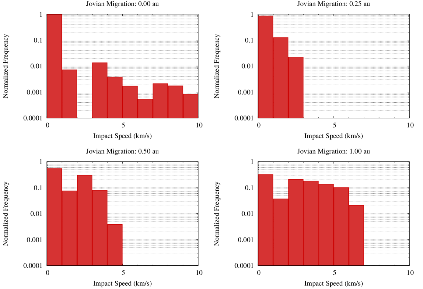
Figure 6: Normalized distribution of the impact velocities of the asteroidal impactors (i.e. the impactors originating between 1 and 4 au in the simulations of Turrini et al. 2011) on Vesta in the four migration scenarios considered in our case study (see Turrini et al. 2011 and Turrini 2014 for more details).
