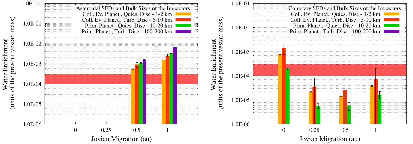
Figure 12: Water accretion experienced by a primordial Vesta with mass similar to that of the present Vesta due to (left) asteroidal impactors and (right) cometary impactors during Jupiter’s mass growth in the different migration scenarios and for the different SFDs considered. For each SFD we report the characteristic diameter of the planetesimals producing the bulk of the impact flux as computed with our Monte Carlo methods. The horizontal regions highlighted in red mark the range of values of Vesta’s water enrichment and represent our upper boundary to Vesta’s water accretion (see Sect. 3 and Stephant et al. 2016a,b; Sarafian et al. 2017a,b). Note that, given that the temporal interval considered in this proof-of-concept study is smaller than the timespan over which Vesta’s crust can be enriched in water, only those scenarios producing water enrichments below the red regions should be considered compatible with present-day Vesta.
