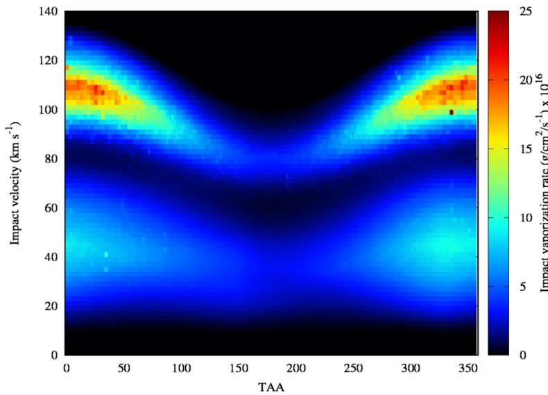
Fig. 25 Total vaporization flux as a function of TAA and the impact velocity. The units are \text{g cm}^{-2} \text{s}^{-1} per 2 \text{ km s}^{-1} bin (Pokorný et al. 2018)
