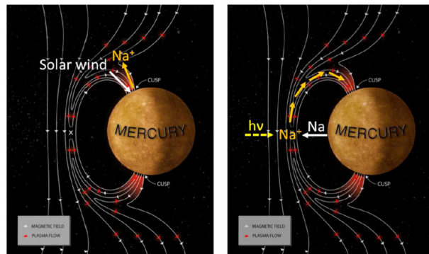
Fig. 27 Two possible sources for \text{Na}^+ ions in the cusp: (left) \text{Na}^+ ions are generated in the cusp, both by solar wind impact and photoionization, and are accelerated by processes there. (Right) Neutral Na atoms are ionized near the magnetopause, picked up in the magnetosheath flow and swept into the cusp. Adapted from Raines et al. (2014)
