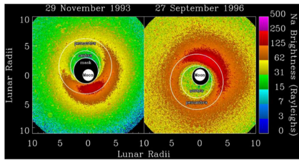
Fig. 10 Observations of Na during two lunar eclipses in 1993 and 1996. A coronagraph mask remains necessary due to refracted light though Earth's atmosphere. Left was taken when the Moon was near the magnetosheath boundary, two days after plasmasheet crossing. Three crossings occurred in such time preceding the image at right, with the last being \sim 4 hours earlier (Mendillo et al. 1999)
