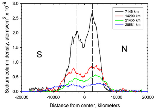
Fig. 9 Cross-tail profiles of Mercury's Na at 110^\circ true anomaly angle. Note the dearth of emission in shadow and the enhancement in the northern lobe, both of which are less pronounced with distance (Potter and Killen 2008)
