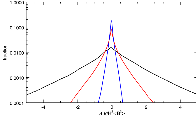
Fig. 8.— Probability distribution functions of the helicity density normalized by H^2 \langle \mathbf{B}^2 \rangle . This corresponds to the average pairwise twist per unit length. Three cases are shown: perfect-gas, symmetric state—black curve; perfect-gas anti-symmetric state—red curve; isothermal case—blue curve. Each curve is computed at a representative time.
