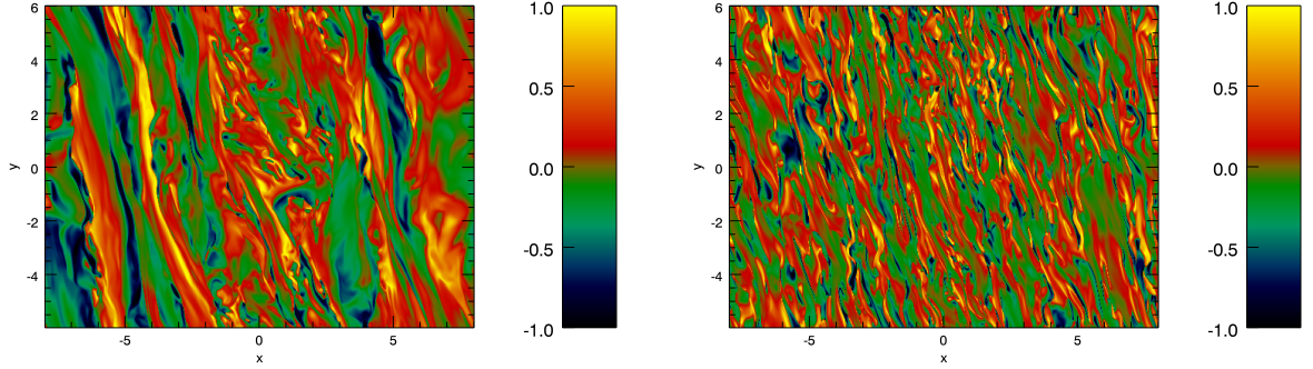
Fig. 7.— Perfect-gas case. Spatial distribution of the normalized helicity density ( \mathbf{A} \cdot \mathbf{B} / |\mathbf{A}| |\mathbf{B}| ) in a horizontal plane at z = 0 at two different times. The left panel corresponds to a representative time in the symmetric state while the right panel corresponds to a representative time in the anti-symmetric state.
