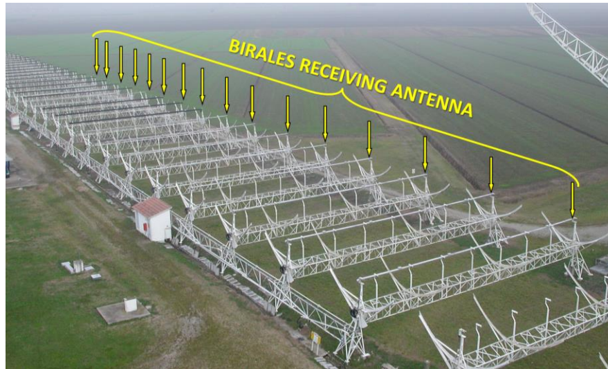
Figure 4: BIRALES receiving antenna
