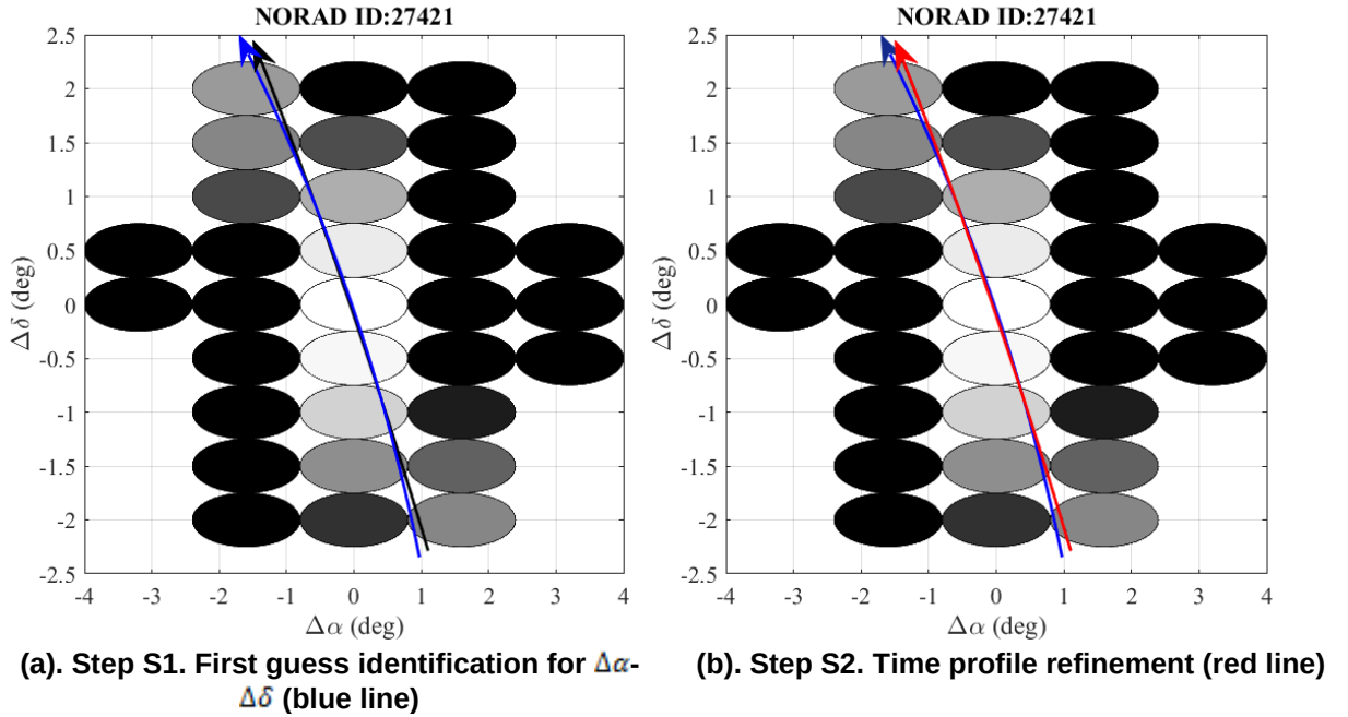
Figure 11: Right ascension and declination profiles definition inside the receiver FoV for object NORAD ID 27421. The black line represents the real track of the object
