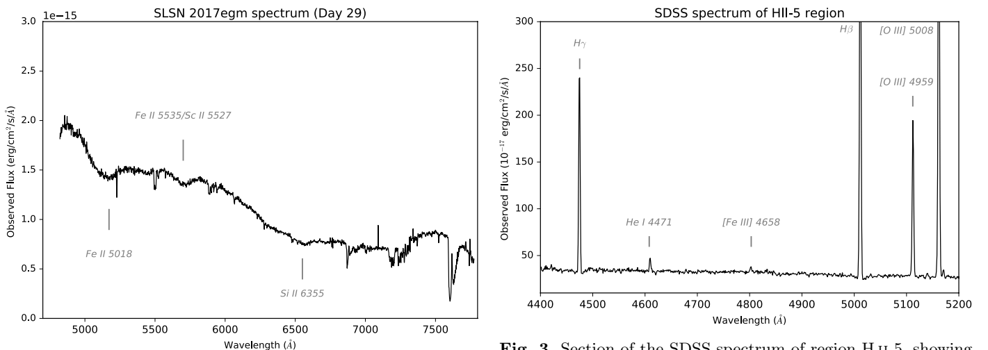
Fig. 2. The observed spectrum of SLSN 2017egm 29 days after discovery, which we use as template for correcting the PMAS data of region H II-4. We identified some typical features of Type-I SLSNe such as Fe II 5018 \lambda , the blend Fe II 5535 \lambda - Sc II 5527 \lambda and Si II 6355 \lambda .
