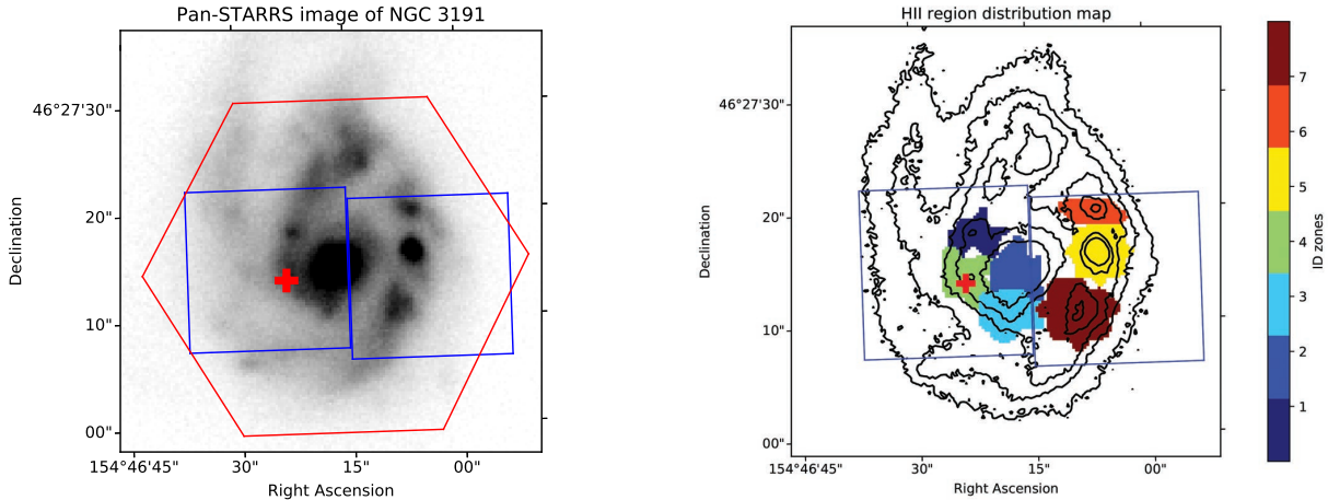
Fig. 1. Left panel: The Pan-STARRS r' -band image of NGC 3191 with the two PMAS fields-of-view (blue squares) and the MaNGA one (red hexagon) superposed. Right panel: Map of the H II regions as obtained with the code described in the text and applied to the PMAS cubes. The SLSN 2017egm position is marked with a red cross in both panels. The levels of the isophotes, from the outermost to the innermost ones, are 21.86, 21.11, 20.66, 20.22 and 19.91 mag/arcsec, respectively.
