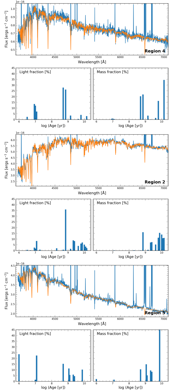
Fig. 10. From top to bottom, the stellar population analysis of the H II regions number 4 (the SLSN region), number 2 (the galaxy centre) and number 5 (the most active region in the galaxy), respectively. Upper panels show the fit to the observed spectral energy distributions, while lower panels show the fraction in luminosity of stellar populations with different ages (left) and their contribution to the total stellar mass (right).
