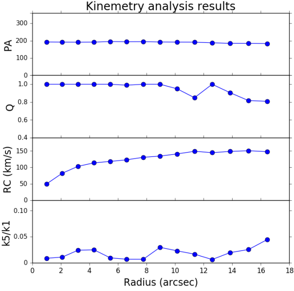
Fig. 9. Best-fit parameters obtained from the kinemetry analysis (Krajnović et al. 2006) for different positions of the tilted-rings relative to the centre of NGC 3191. From the top: Position angle in degrees, the ellipticity parameter q , the rotation curve (RC) that corresponds to the first order k1 of the harmonic expansion corrected for the inclination of the galaxy, and the k5/k1 ratio.
