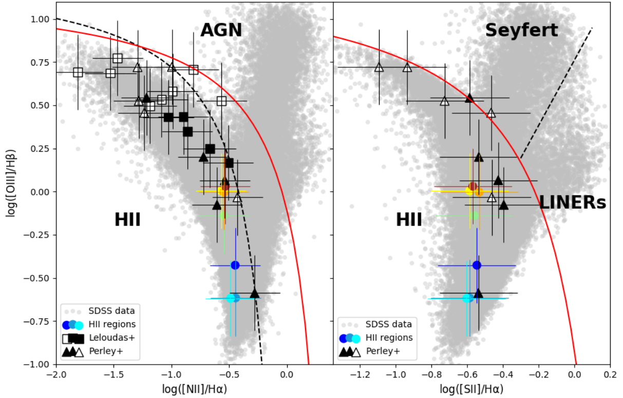
Fig. 5. The BPT emission-line diagnostic used to distinguish the ionization mechanism acting in the nebular gas in galaxies. Two distinct diagnostics are used here: the left side shows [\text{O III}] 5008 \text{ \AA} / \text{H}\beta versus [\text{N II}] 6584 \text{ \AA} / \text{H}\alpha , while the right side shows the [\text{S II}] 6718/32 \text{ \AA} doublet instead of [\text{N II}] . The solid red curves in both panels denote the theoretical demarcation line between AGNs and star-forming galaxies proposed by Kewley et al. (2001). In the left panel, the black dashed curve corresponds to the empirical demarcation between AGNs and SF-galaxies proposed by Kauffmann et al. (2003), while in the right panel the black dashed line marks the division between active Seyfert galaxies and LINERs proposed by (Kewley et al. 2006). Grey data points are taken from the SDSS DR7 sample of galaxies described in Tremonti et al. (2004). Coloured circles correspond to the H II regions described in the text with the same colour coding used in Fig. 1. Squares and triangles represent SLSN-host data from Leloudas et al. (2015) and Perley et al. (2016), empty symbols represent H-poor SLSNe, filled ones H-rich SLSNe. The SLSN 2017egm location (light-green circle) shows it is one of the most metal-rich Type-I SLSN.
