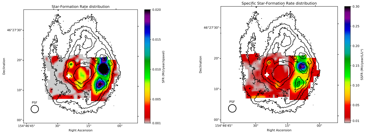
Fig. 4. Left panel: SFR map in the galaxy for the two fields covered by PMAS observations, computed using the Kennicutt (1989) diagnostic. Right panel: The specific SFR obtained by weighting the SFR map and the rest-frame B -luminosity map, applying the same method described in Christensen et al. (2004). The dimensions of each spaxel have been interpolated in the figure, showing elements of 0.25 \times 0.25 arcsec. The SLSN position is marked with a white cross.
