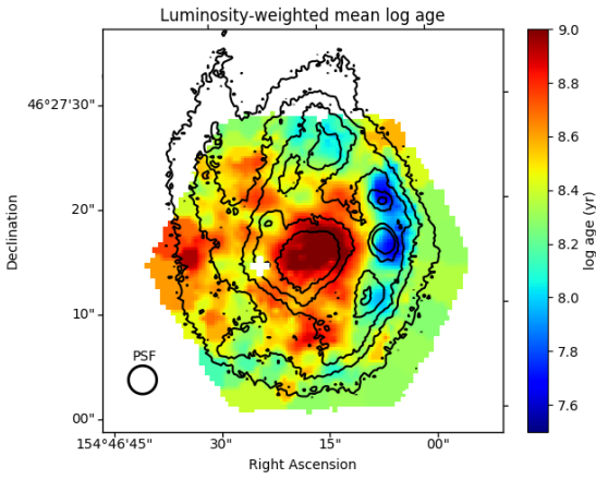
Fig. 11. The luminosity weighted (log) age distribution estimated with the STARLIGHT code, following the prescriptions given in Cid Fernandes et al. (2013). The location of SLSN 2017egm is reported with a black cross while the location of PTF10bgl is reported with a black circle.
