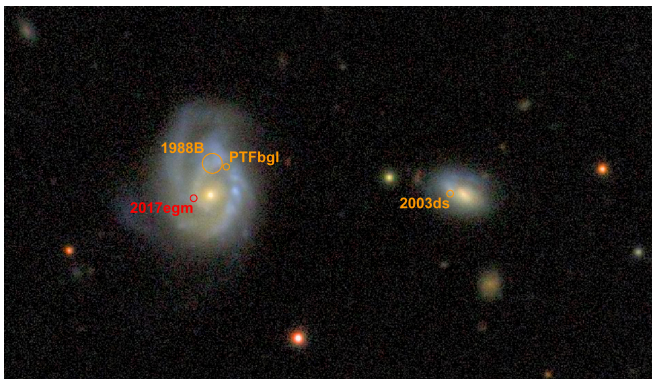
Fig. 7. Colour image of NGC 3191 and its neighbour MCG+08-19-017 created combining multiband data from the PanSTARRS and the SDSS image catalogues. We also mark the locations of all four SNe that occurred in this galaxy pair. North is up and East is to the left, the field of view is 3/2 \times 1/8 .
