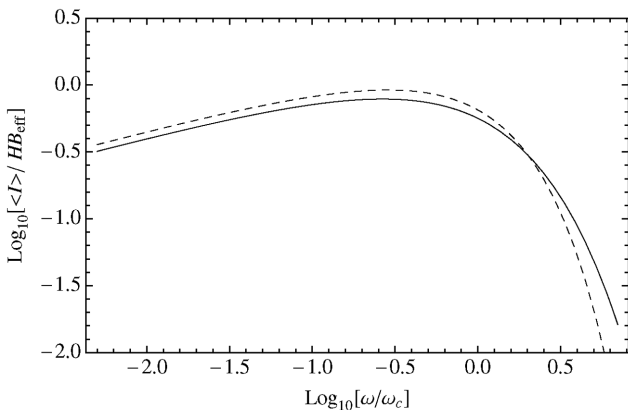
Figure 6. Comparison of the spectral profile of the synchrotron emissivity from a mono-energetic particle distribution, both for a completely ordered MF (dashed line) and a fully random MF (solid line). B_{\text{eff}} indicates the effective MF for each case, namely \bar{B} in the former case and \sqrt{2}\sigma in the latter.
