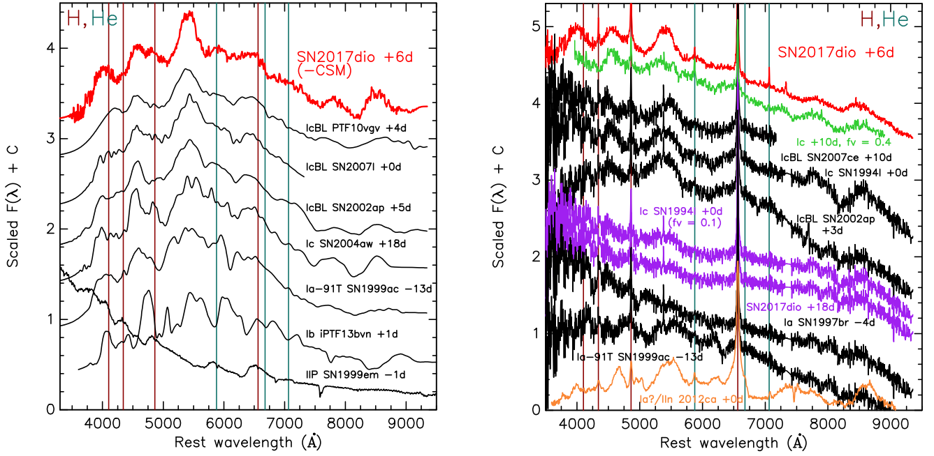
Figure 3. (Left) Comparison of the CSM interaction-subtracted spectrum of SN 2017dio (red) with spectra of other SNe (black; including SNID templates of Modjaz et al. 2014). (Right) Comparison of the +6 day spectrum of SN 2017dio (red) with those of other SNe combined with interaction spectrum (black; f_V = 0.3 ), a template SN Ic+CSM interaction spectrum from Leloudas et al. (2015, green), and SN 2012ca (orange). The spectrum of SN 1994I combined with the interaction spectrum ( f_V = 0.1 ) is shown for comparison with SN 2017dio at +18 days. The comparison spectra are from WiSeREP. In both panels, phases are days from maximum for spectra other than SN 2017dio.
