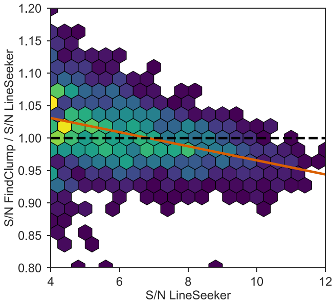
Figure 4. Density map of the ratio between the S/N values obtained with FindClump and LineSeeker of an artificial/simulated data cube. The color of the cells follows a logarithmic scale proportional to the number of points in each cell. The solid orange line corresponds to a linear fit to the points with a 7% slope showing that the S/N values obtained with FindClump are slightly higher than the ones obtained with LineSeeker for the fainter sources.
