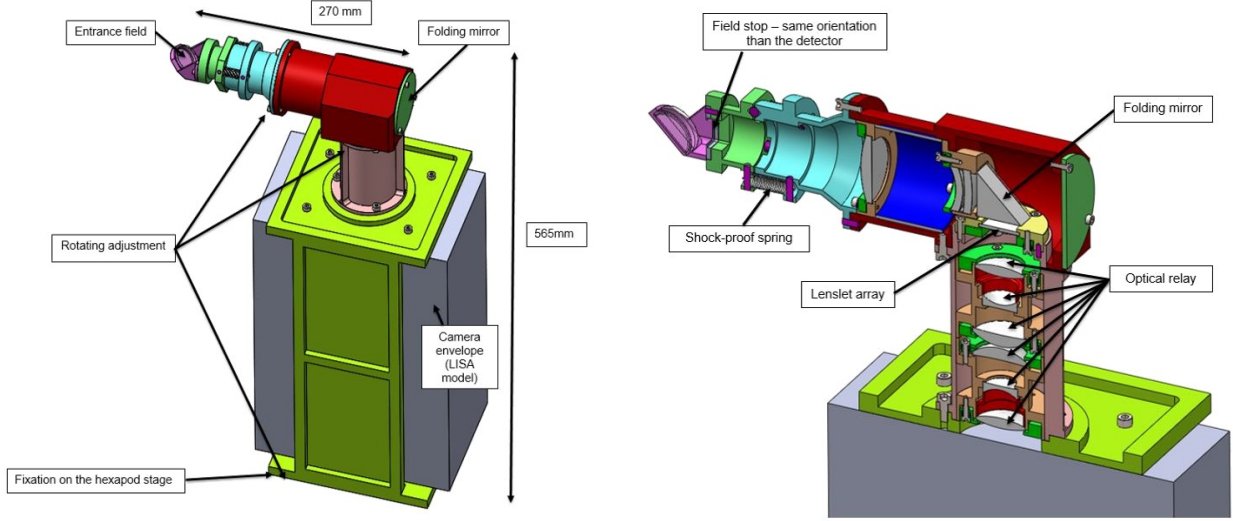
Figure 5. LGS WFS probe opto-mechanical design.
