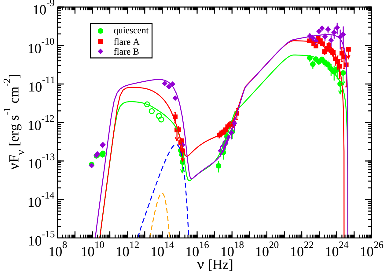
Fig. 3.— Broadband SED model for PKS 2326–502. The data are modeled with a one-zone leptonic model of blazar emission (Finke et al. 2008). The low-energy component is modeled as a combination of synchrotron emission from the jet and thermal emission from the accretion disk. A double broken power law is used to model the electron distribution during the quiescent state flare A. A change in the size of the emitting region is used to model flare B. The smaller dashed green curve represents emission from the dust torus and the larger dashed blue curve is accretion disk emission. The high-energy component is explained by inverse Compton scattering of dust torus photons by electrons within the jet. Hollow circles represent non-simultaneous data.
