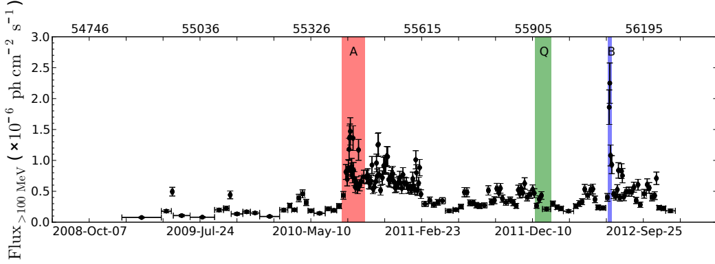
Fig. 1.— Fermi -LAT adaptively binned \gamma -ray light curve in the 100 MeV to 300 GeV energy range for PKS 2326–502. It covers the period from 2009 February 21 (MJD 54883) to 2012 December 05 (MJD 56266). The bin sizes are set such that a constant flux uncertainty of 15% is maintained. Three different states of the source are selected and their MWL SEDs are modeled. The long active state is from 2010 July 31 - 2010 September 29 (flare A, in red), the quiescent state from 2011 December 18 through 2012 January 29 (period Q, in green), and a short, high peaked, flaring state from 2012 June 25 through 2012 July 05 (flare B, in purple).
