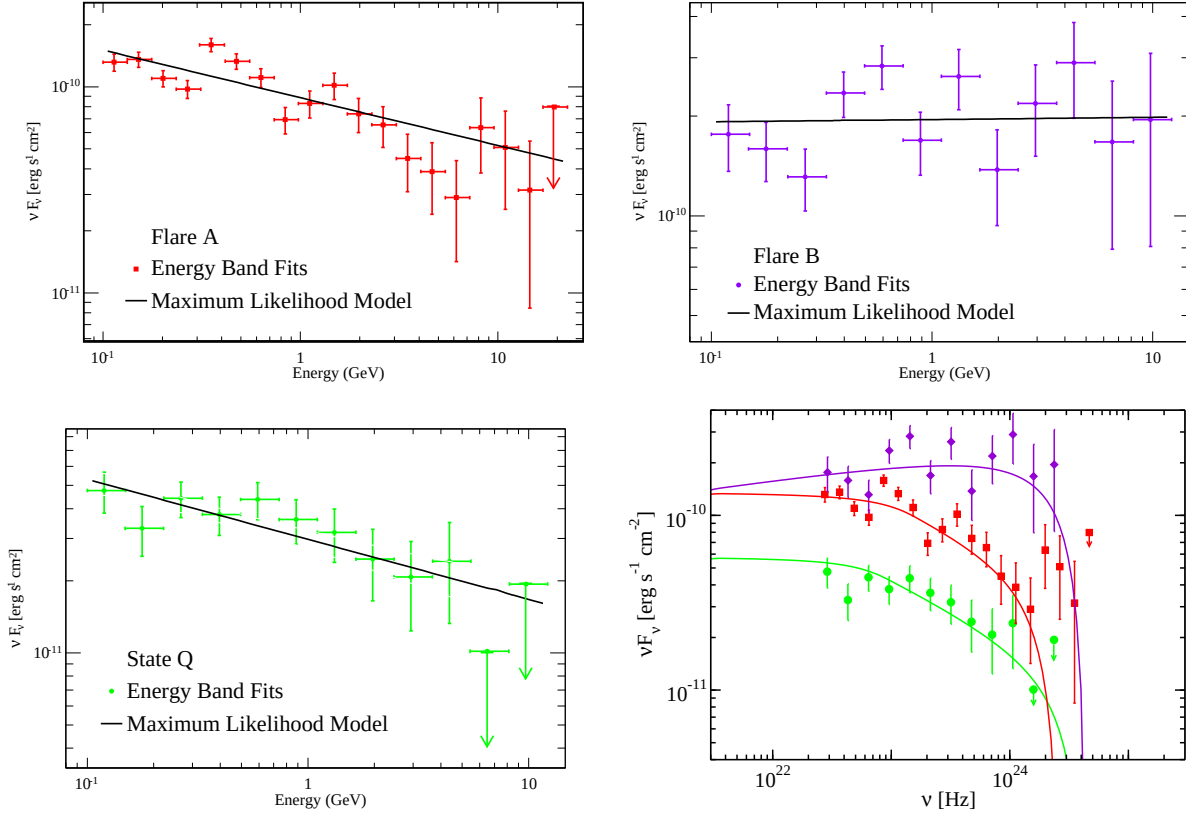
Fig. 2.— \gamma -ray SEDs of PKS 2326–502. The top left plot shows the SED during flare A. Top right is flare B. Bottom left is period Q. The black line on each plot shows the power-law fit. The bottom right plot shows all three states plotted together. The green, red and purple points represent the quiet, A, and B states respectively. Note that the solid lines on the bottom right figure are the SED models, not fits to the data.
