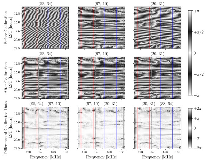
Figure 6. Effect of calibration on the phases of visibilities from three redundantly spaced 14.7 m baselines; mn polarization. The antenna numbers refer to those given in Figure 3. The color scale is cyclic; black is \pm\pi/2 and white is 0 and \pm\pi . The extent of the low band is indicated with red lines and the high band is shown with blue lines. Top row: before calibration. Middle row: after calibration. Bottom row: the three pairs of differences of the calibrated phases. Note that the agreement between baselines is excellent near the Galactic Center but shows significant differences at some other times.
